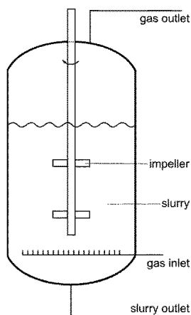
Figure 1: Exemplary vessel used in present invention.
