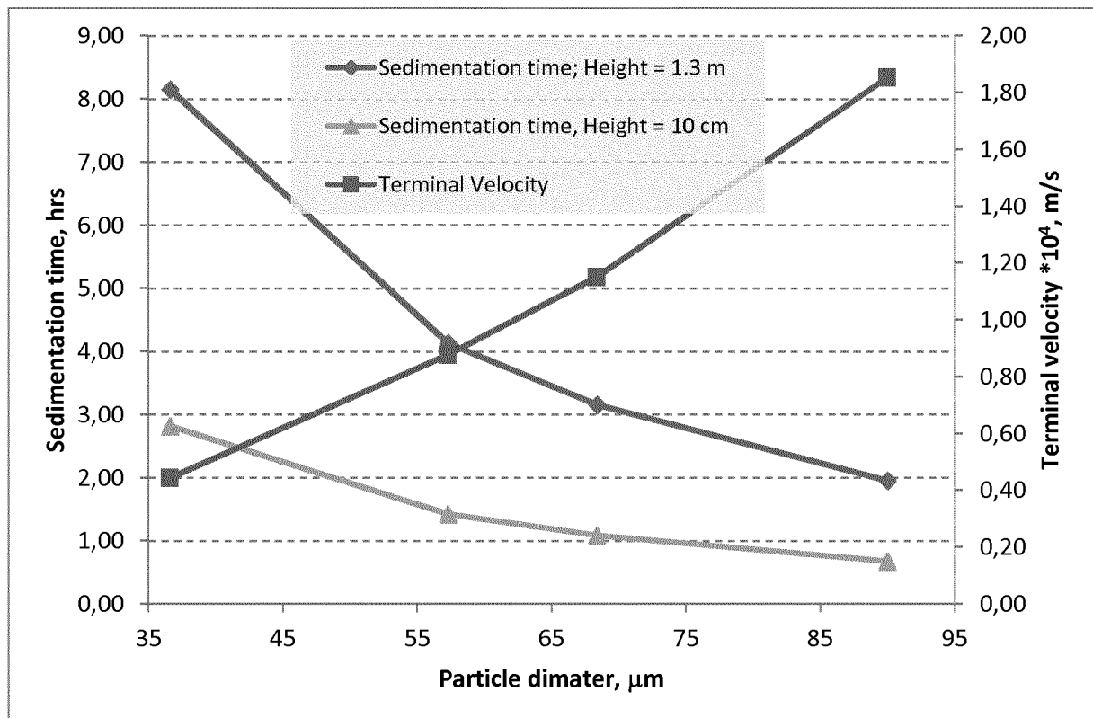
5 Figure 2: Sedimentation time for different particles average diameters along the whole height of the vessel (Example 1).
