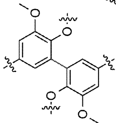
5-5 (3-27%)
