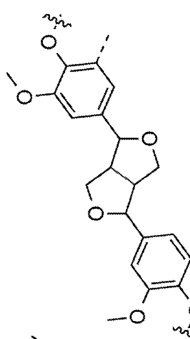
\beta - \beta (2-12%)
