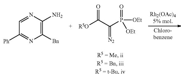
Scheme 4. Synthesis of Intermediates A-C
