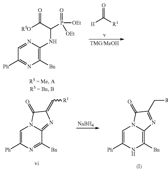
Scheme 2. Synthesis of the compound of formula (I)
