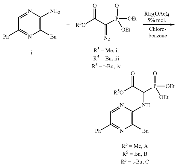
Scheme 1. Synthesis of intermediates A-C
