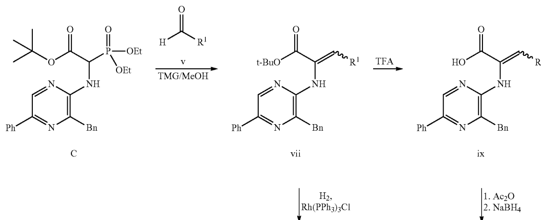
Scheme 3. Synthesis of the compound of formula (I)
