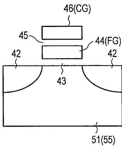
Memory cell MC
