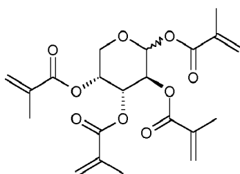
RM-28
