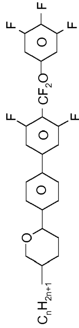
ACQU-n-F
