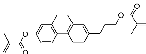
RM-8
