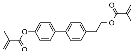
RM-2
