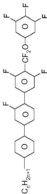
PPGU-n-F
