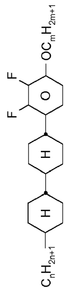
CCP-Vh-m
