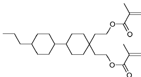
RM-20
