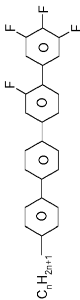
PPGU-n-F
