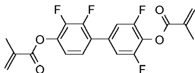
RM-5
