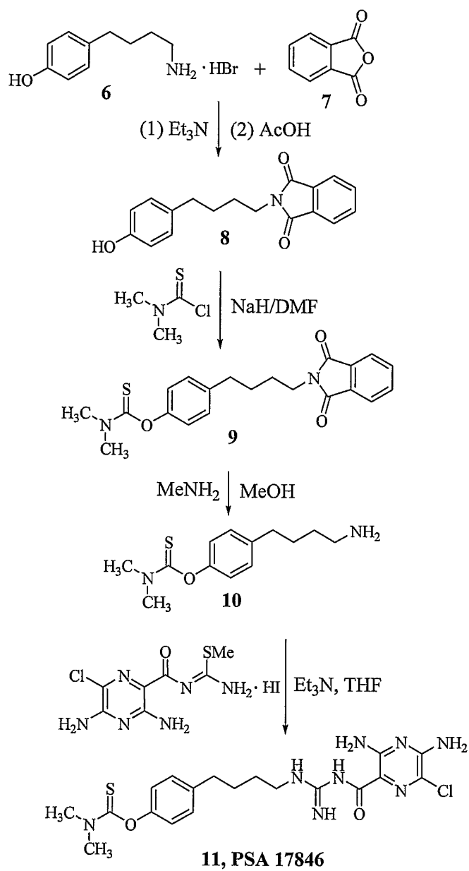
Scheme 2. Synthesis of PSA 17846
