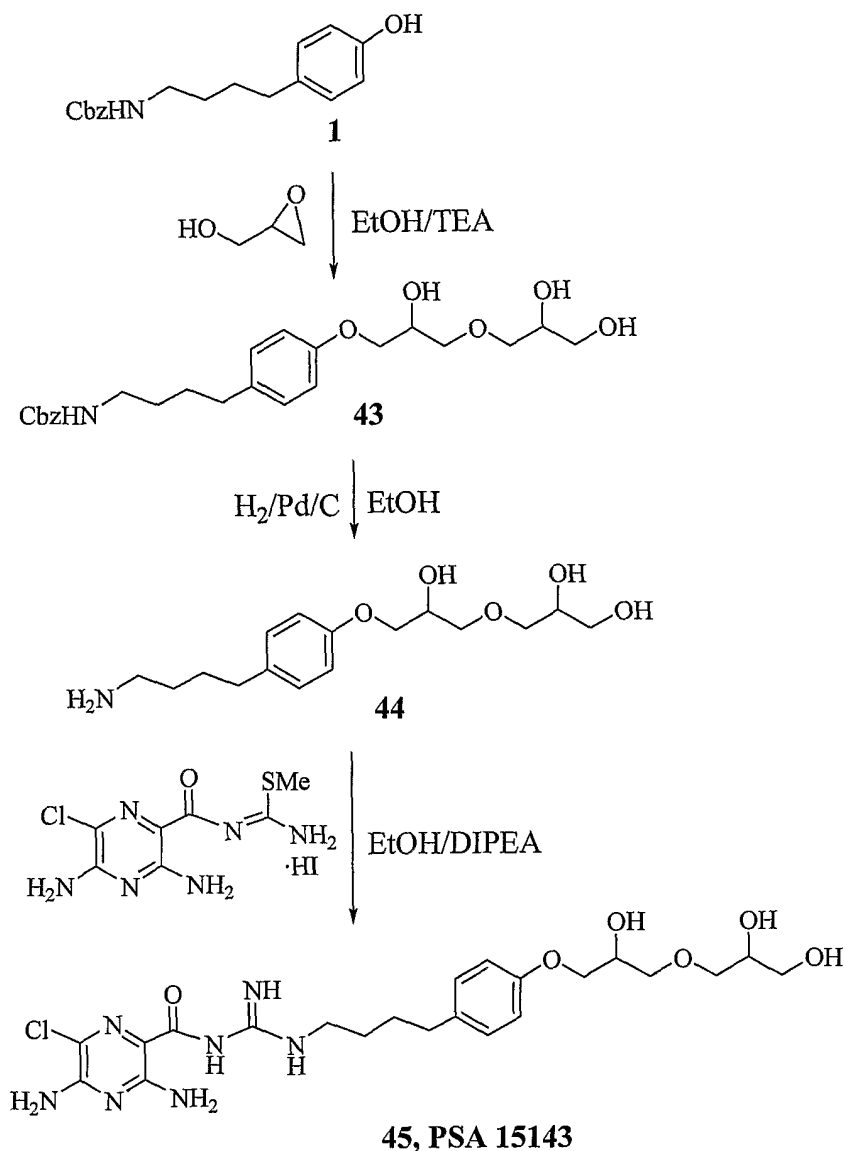
Scheme 11. Synthesis of PSA 15143
