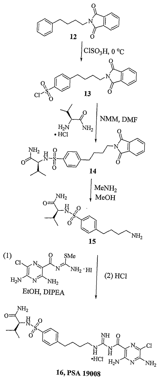
Scheme 3. Synthesis of PSA 19008
