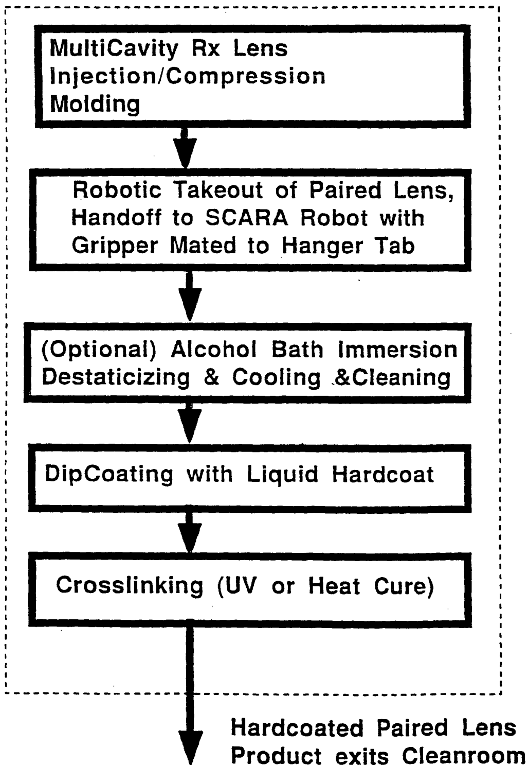
Figure 4B: Automated "Mold and Dipcoat" ("Continuous Process")
