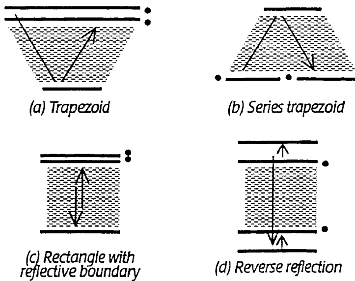
Fig. 18 - Example touch region boundaries
