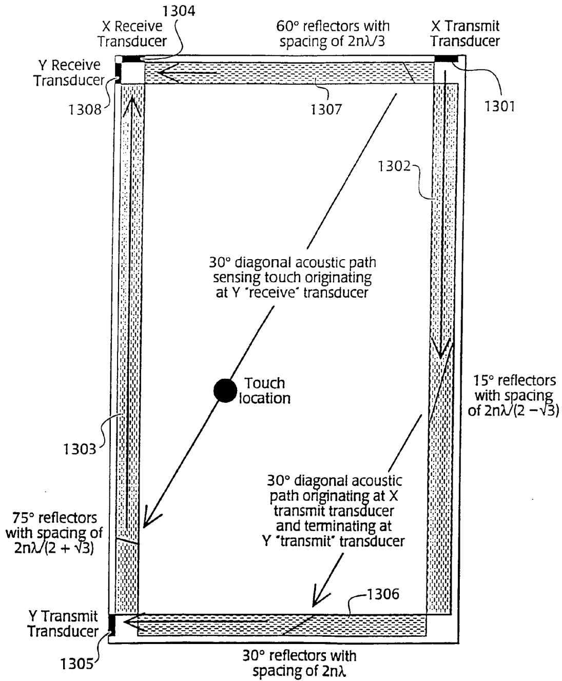
Figure 14 - V Subsystem of X,Y,U,V Sensor
