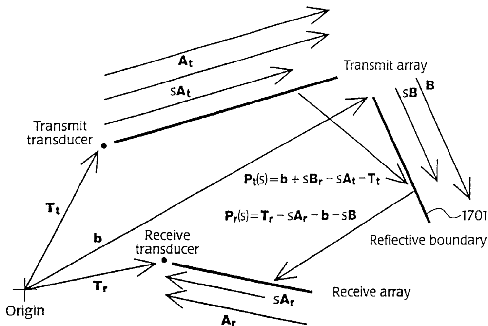
Fig. 17 - Coordinate subsystem with scattering
