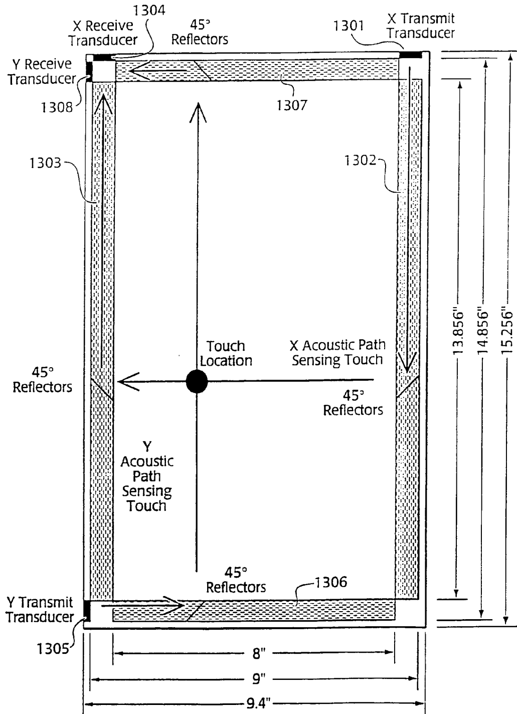
Figure 13 - X, Y, 30° Sensor: (a) X & Y Subsystems
