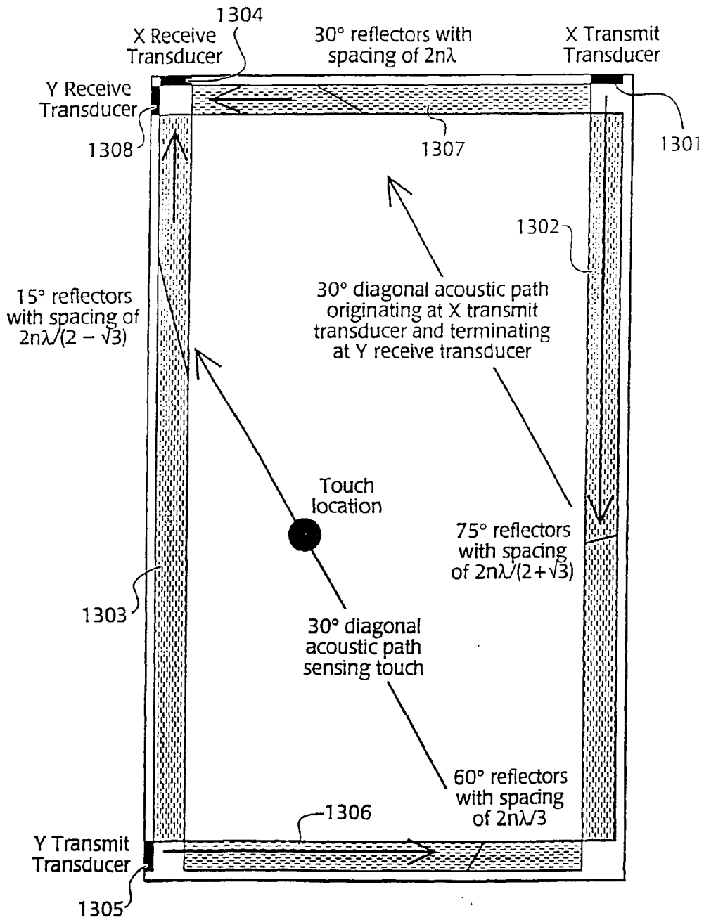
Figure 13 - X, Y, 30° Sensor: (b) Diagonal Subsystems
