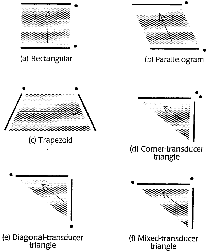
Fig. 12 - Example touch region geometries
