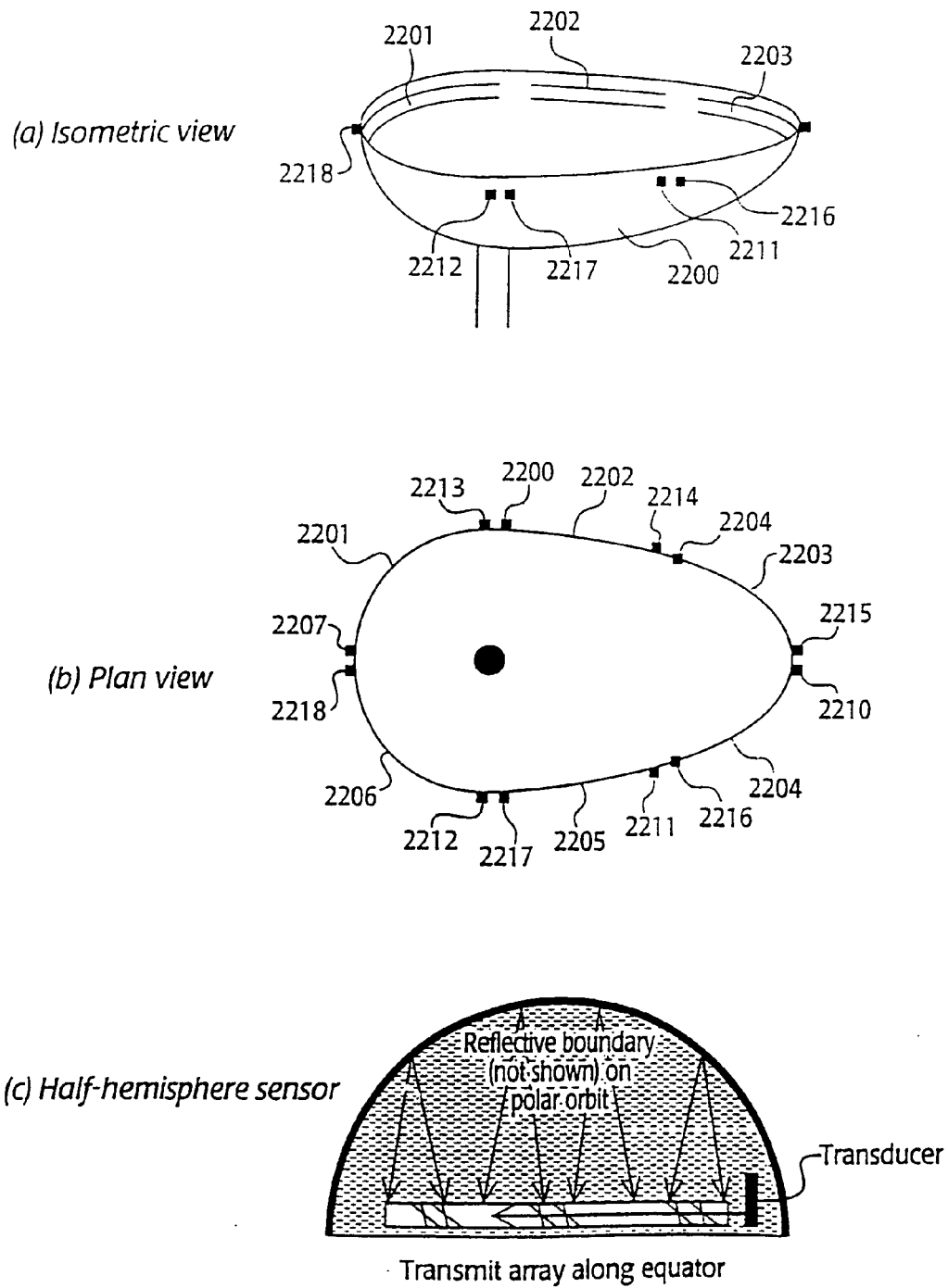
Fig. 22 - Basin sensor
