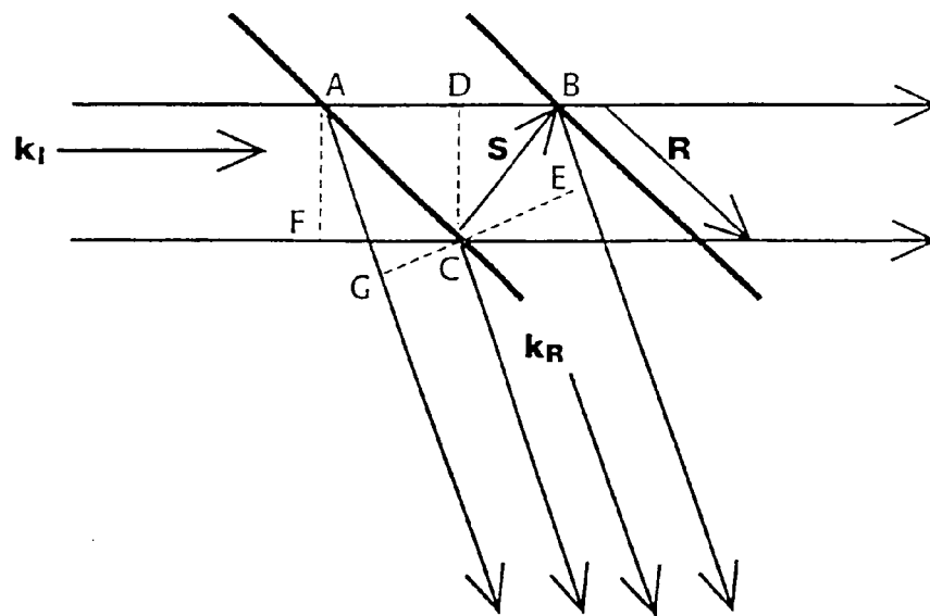
Fig. 11 - Array reflector spacing and orientation
