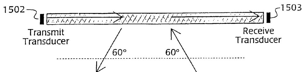
(a) Reflective array detail
