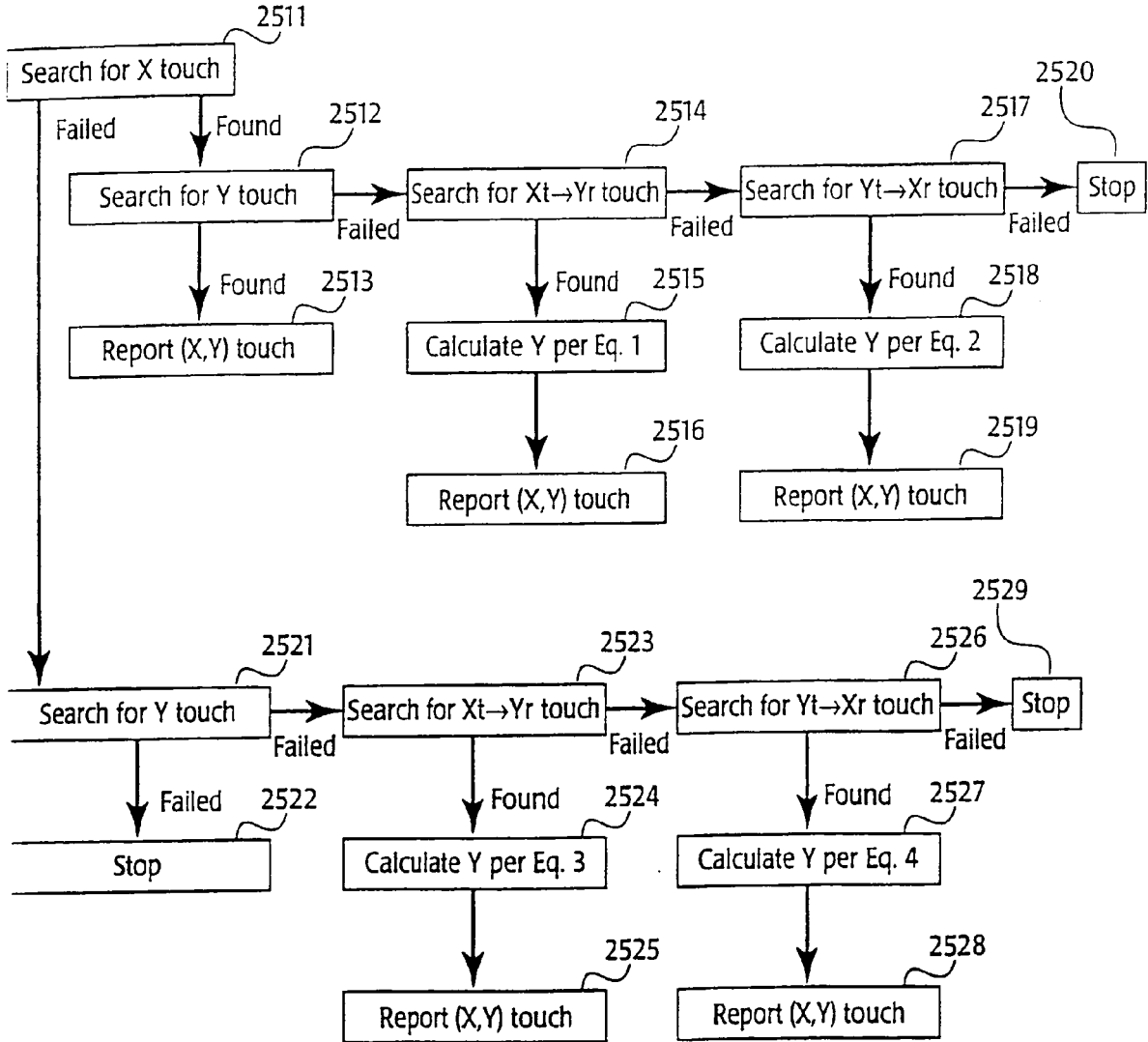
Fig. 25(b) Anti-Shadowing Algorithm Flow Chart
