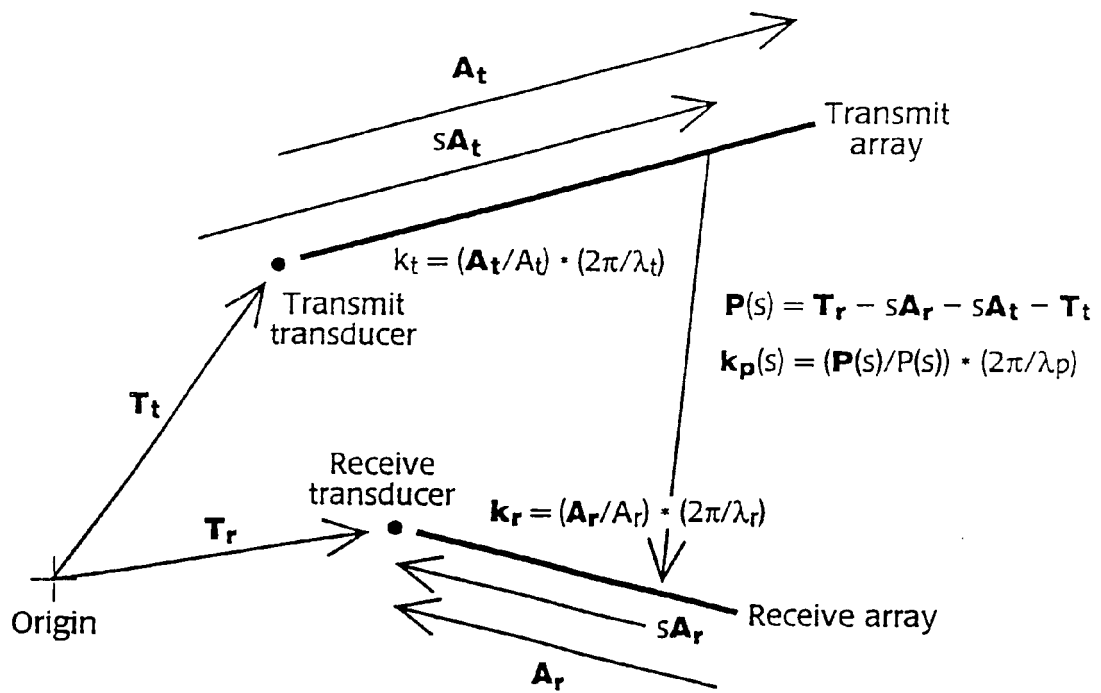
Fig. 10 - Planar coordinate subsystem
