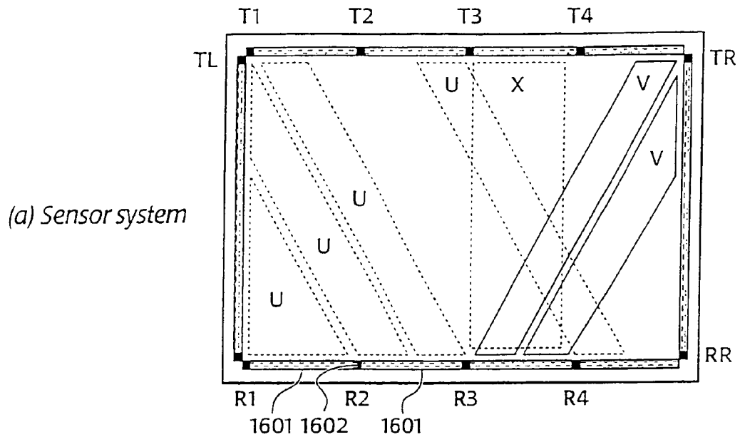
Fig. 16 - Large rectangular sensor
