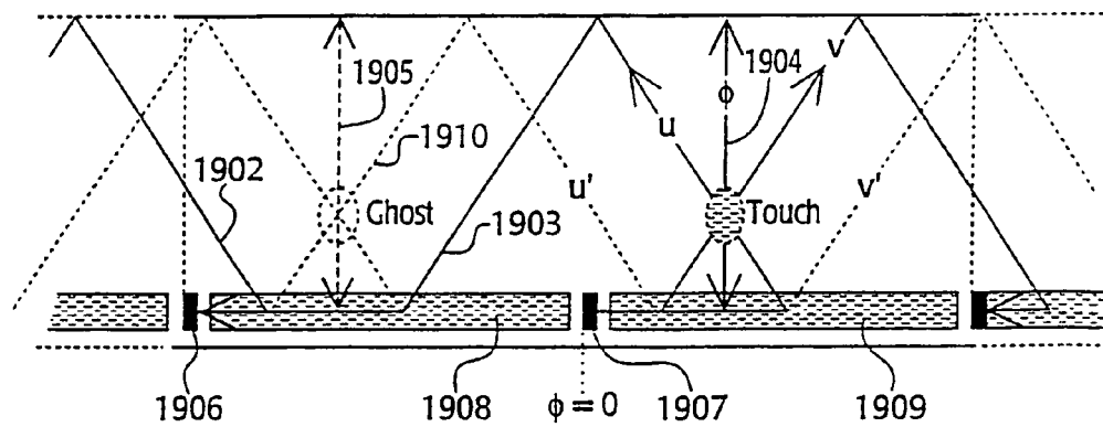
(b) "Planar" sensor with periodic extensions
