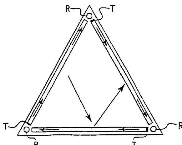
(c) Triangular sensor geometry
