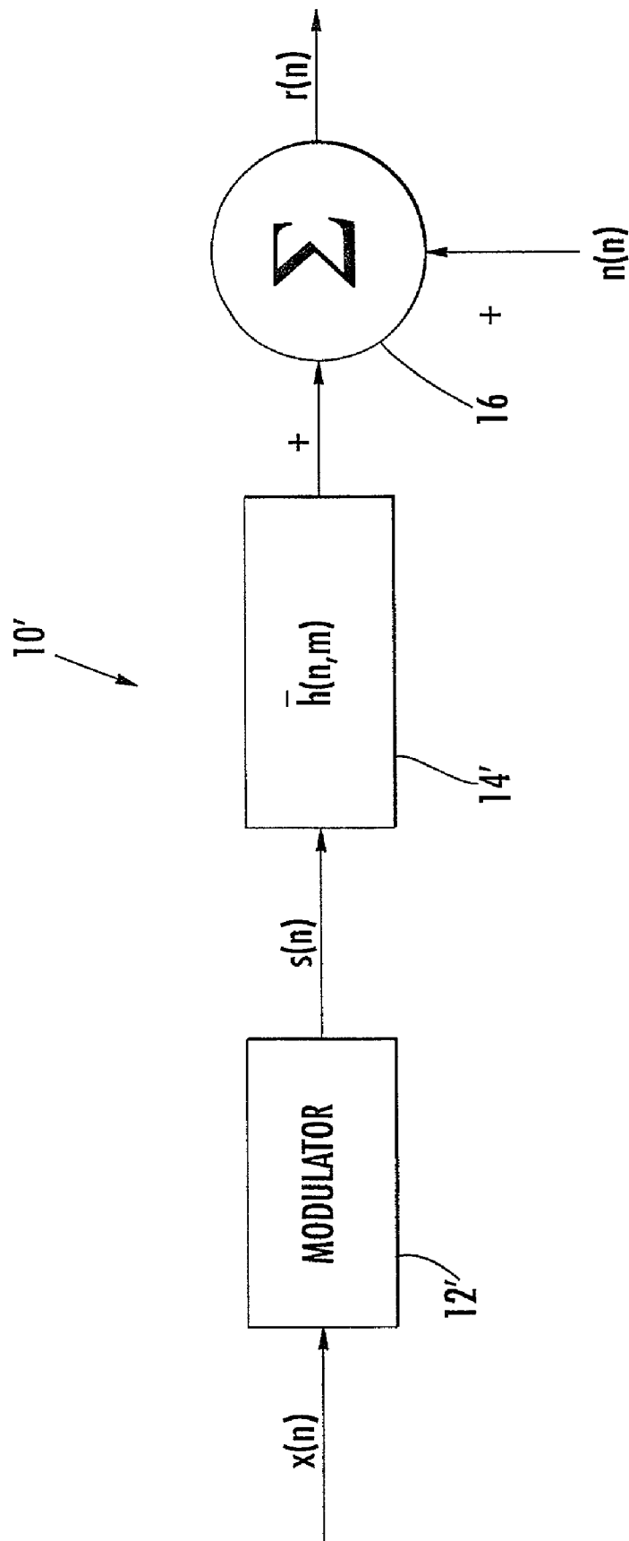
FIG. 5. (PRIOR ART)
