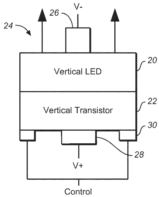
FIG. 2 (PRIOR ART)
