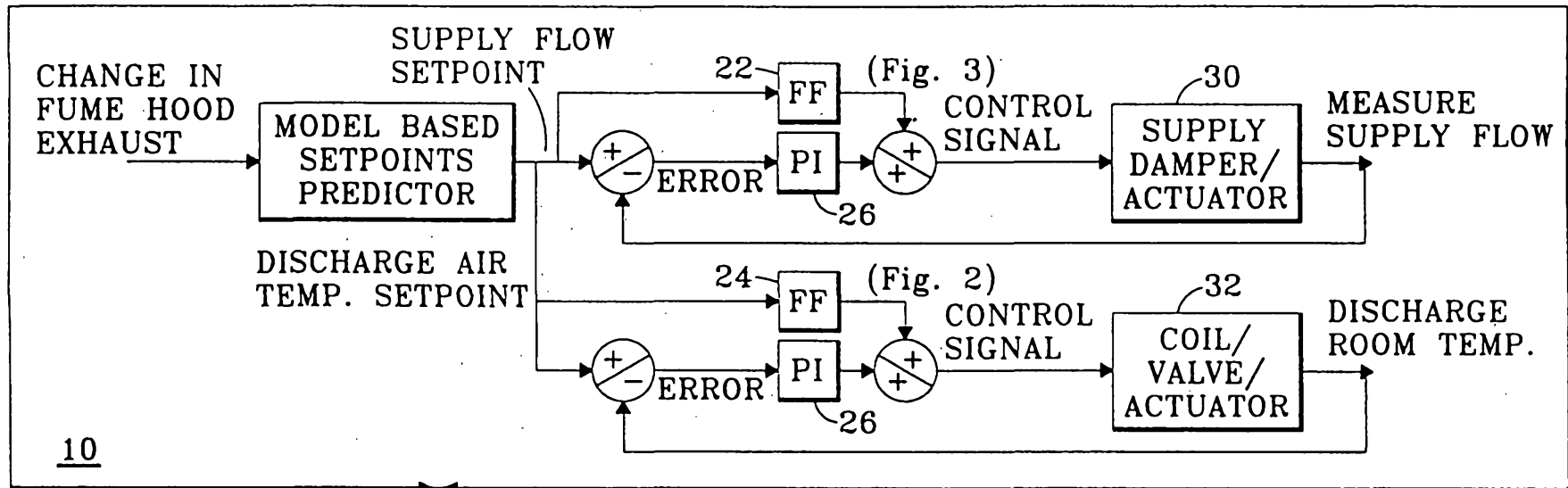
TEMPERATURE CONTROL-HEATING
