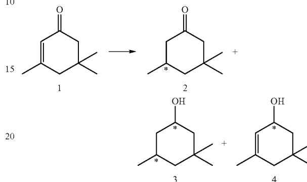
Scheme A: Asymmetric hydrogenation of isophorone 1
