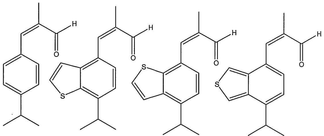
cyclamenaldehyde
