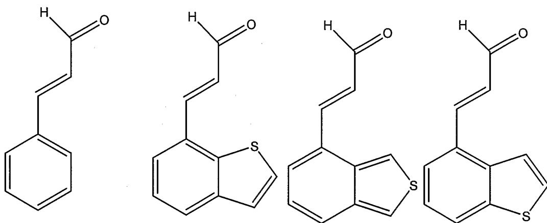
cinamaldehyde
