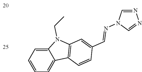
compound XXVII
