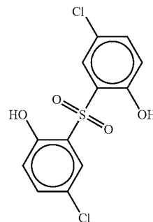
Compound XLII
