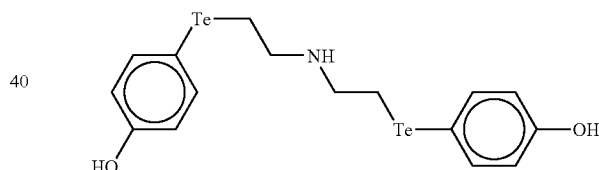
Compound XLV
