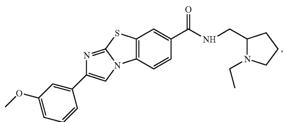
Compound XXI
