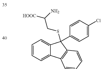
compound XXXIX
