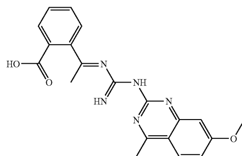
compound XXVI
