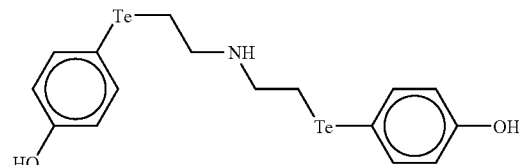
Compound XLV
