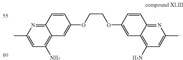
compound XLIII
