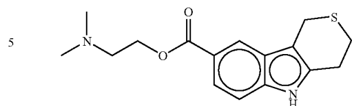
compound XXXII
