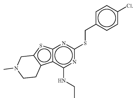
compound XXIII
