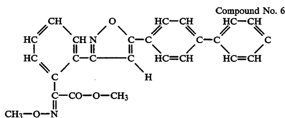
(Z)-methyl 2-methoxyimino-2-[2-(5-(4-phenylphenyl)isooxazol-3-yl]phenyl]acetate; and furthermore, the following compounds:
