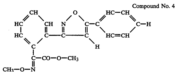
(Z)-methyl 2-methoxyimino-2-[2-(5-phenyl)isooxazol-3-yl]phenylacetate.
