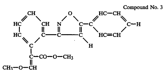
(Z)-methyl 3-methoxy-2-[2-(5-phenyl)isooxazol-3-yl]phenylacrylate.
