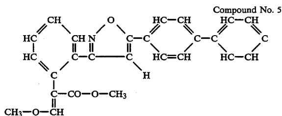
(Z)-methyl 3-methoxy-2-[2-(5-(4-phenylphenyl)isooxazol-3-yl]phenyl]acrylate.
