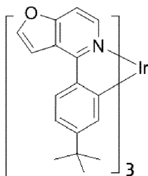
Organic metal compound (IX)
