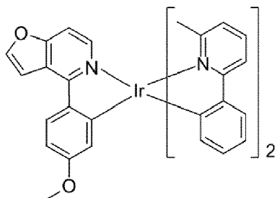
Organic metal compound (XLI)
