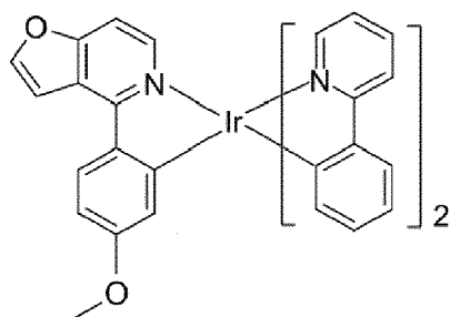
Organic metal compound (XXX)
