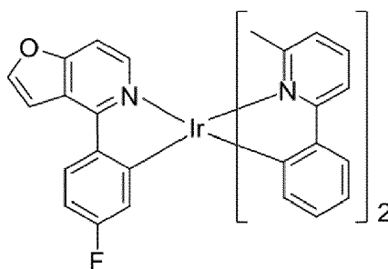
Organic metal compound (XL)
