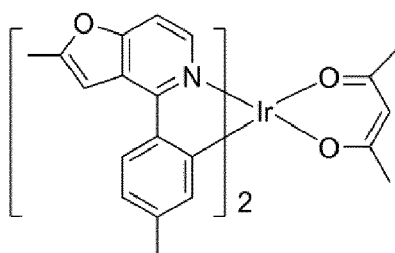
Organic metal compound (XVII)
