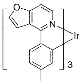
Organic metal compound (X)
