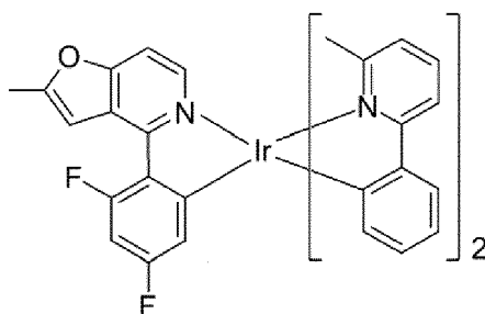
Organic metal compound (XXXIX)
