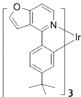
Organic metal compound (IX)
