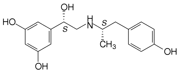
(S,S)-Fenoterol
