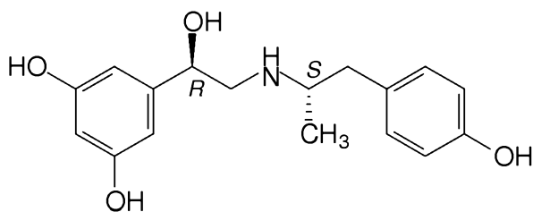
(R,S)-Fenoterol
