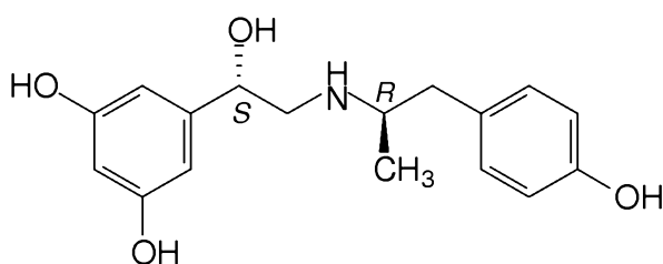
(S,R)-Fenoterol
