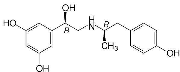
( R,R )-Fenoterol
