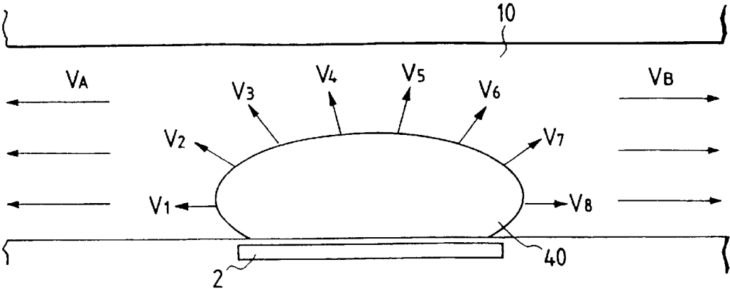
FIG. 3 PRIOR ART
