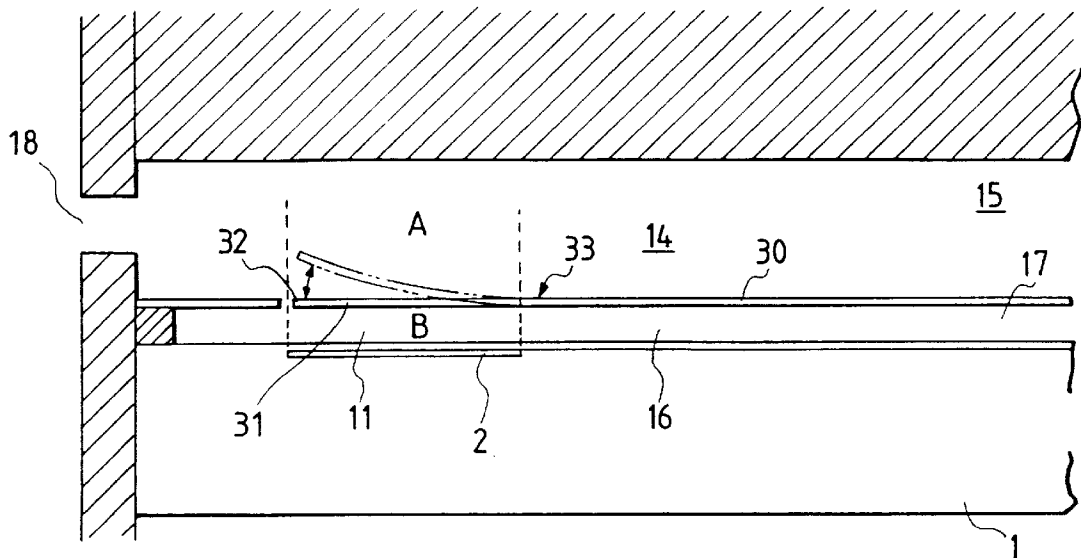
FIG. 6 PRIOR ART
