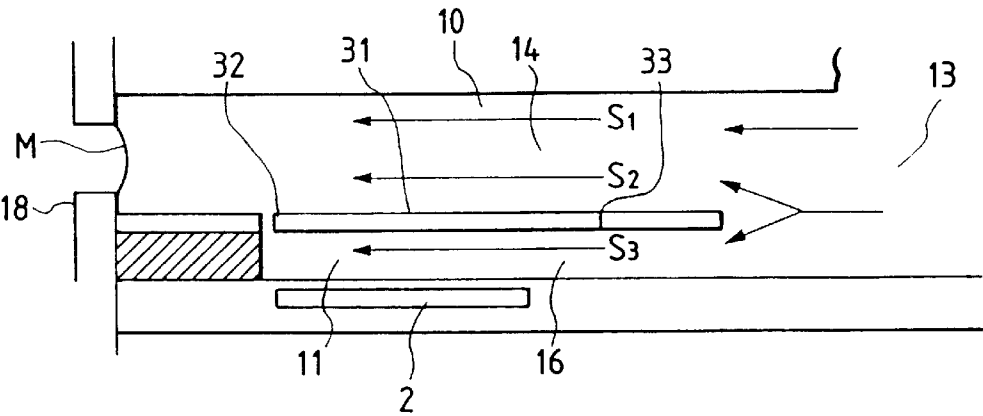
FIG. 5 PRIOR ART
