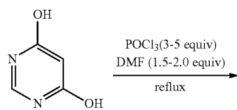
Scheme 15
