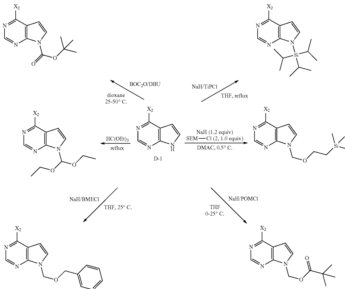
Scheme 13
