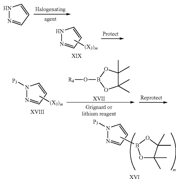
Scheme 14
