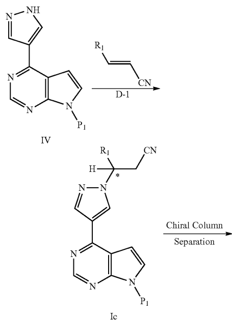
Scheme 6
