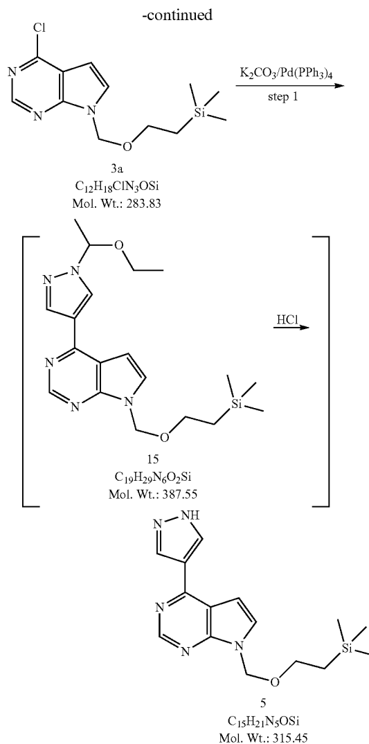
4-(1H-Pyrazol-4-yl)-7-(2-trimethylsilanylethoxymethyl)-7H-pyrrolo[2,3-d]pyrimidine (5)
