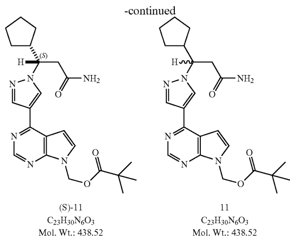
(4-(1-(3-Amino-1-cyclopentyl-3-oxopropyl)-1H-pyrazol-4-yl)-7H-pyrrolo[2,3-d]pyrimidin-7-yl)methyl pivalate (11)
