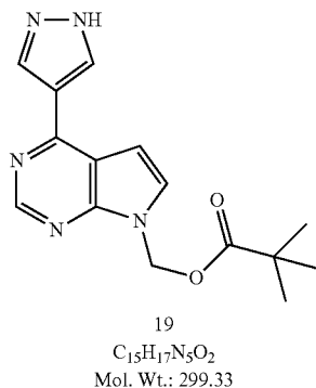
[4-(1H-Pyrazol-4-yl)-7H-pyrrolo[2,3-d]pyrimidin-7-yl]methyl pivalate (19)
