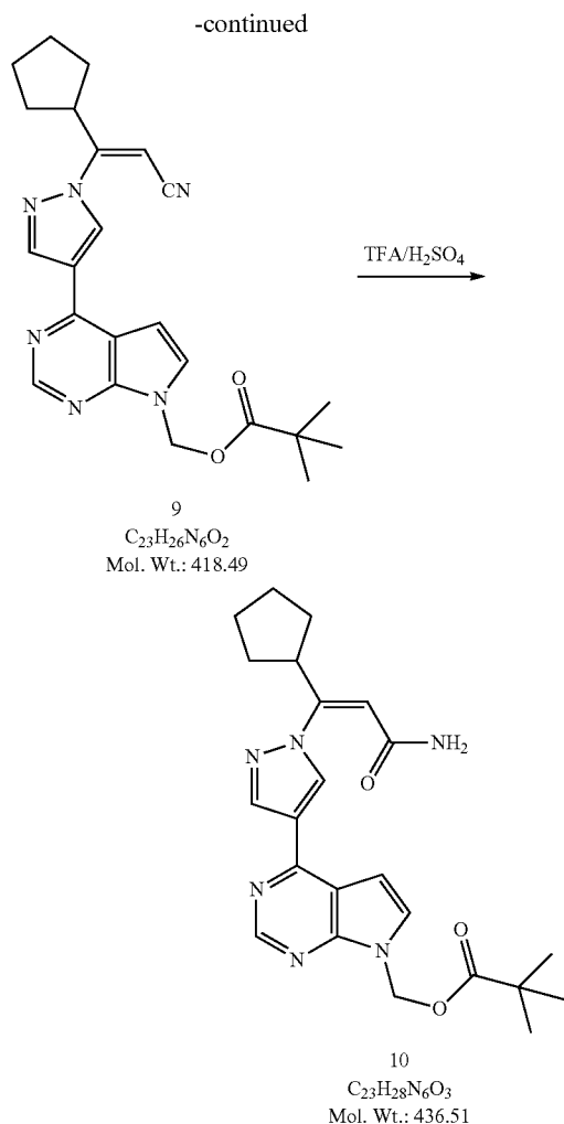
4-(1-(2-Cyano-1-cyclopentylvinyl)-1H-pyrazol-4-yl)-7H-pyrrolo[2,3-d]pyrimidin-7-ylmethyl pivalate (9)
