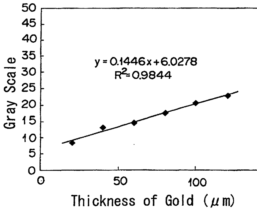
Calibration Curve of Gold (AB Pectoral Average)
