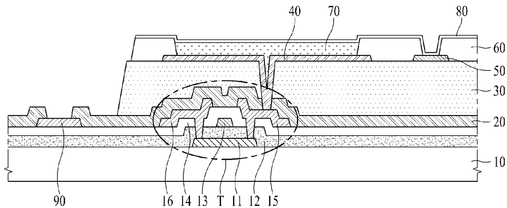
FIG. 1 (RELATED ART)
