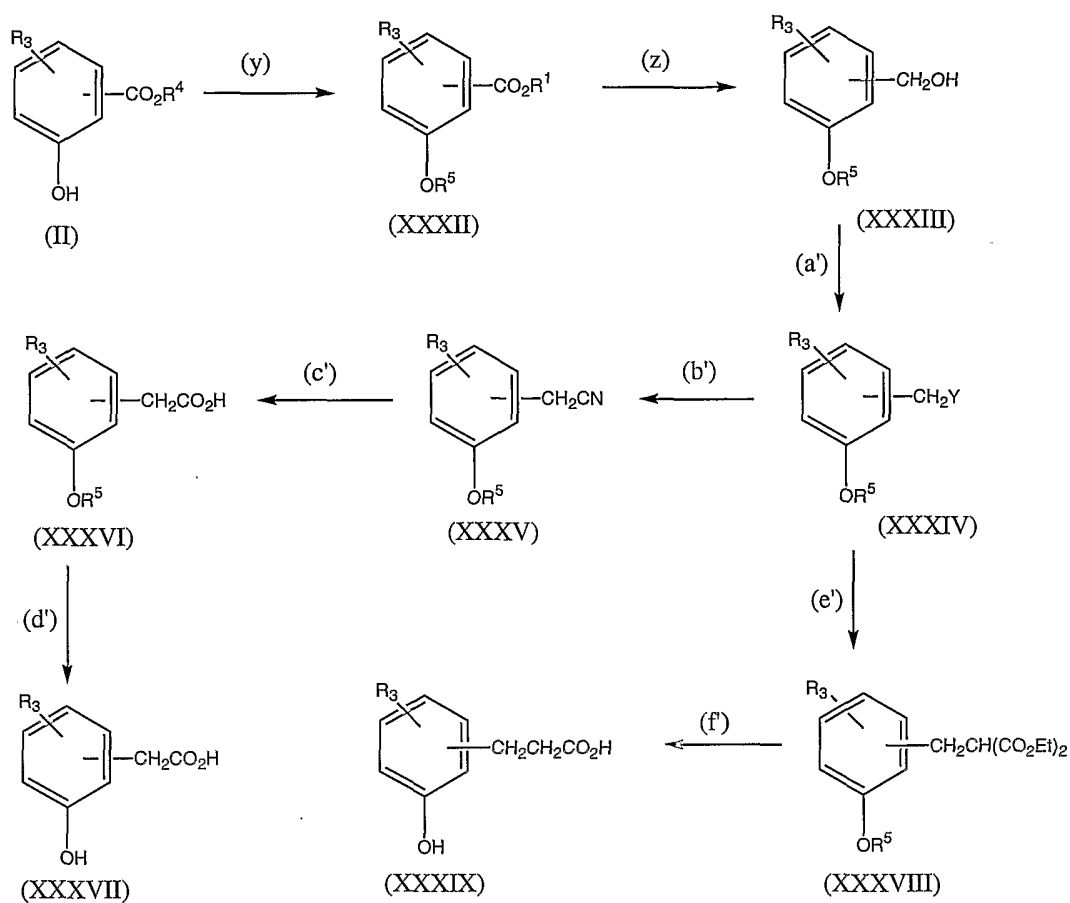
Reaction Scheme 8
