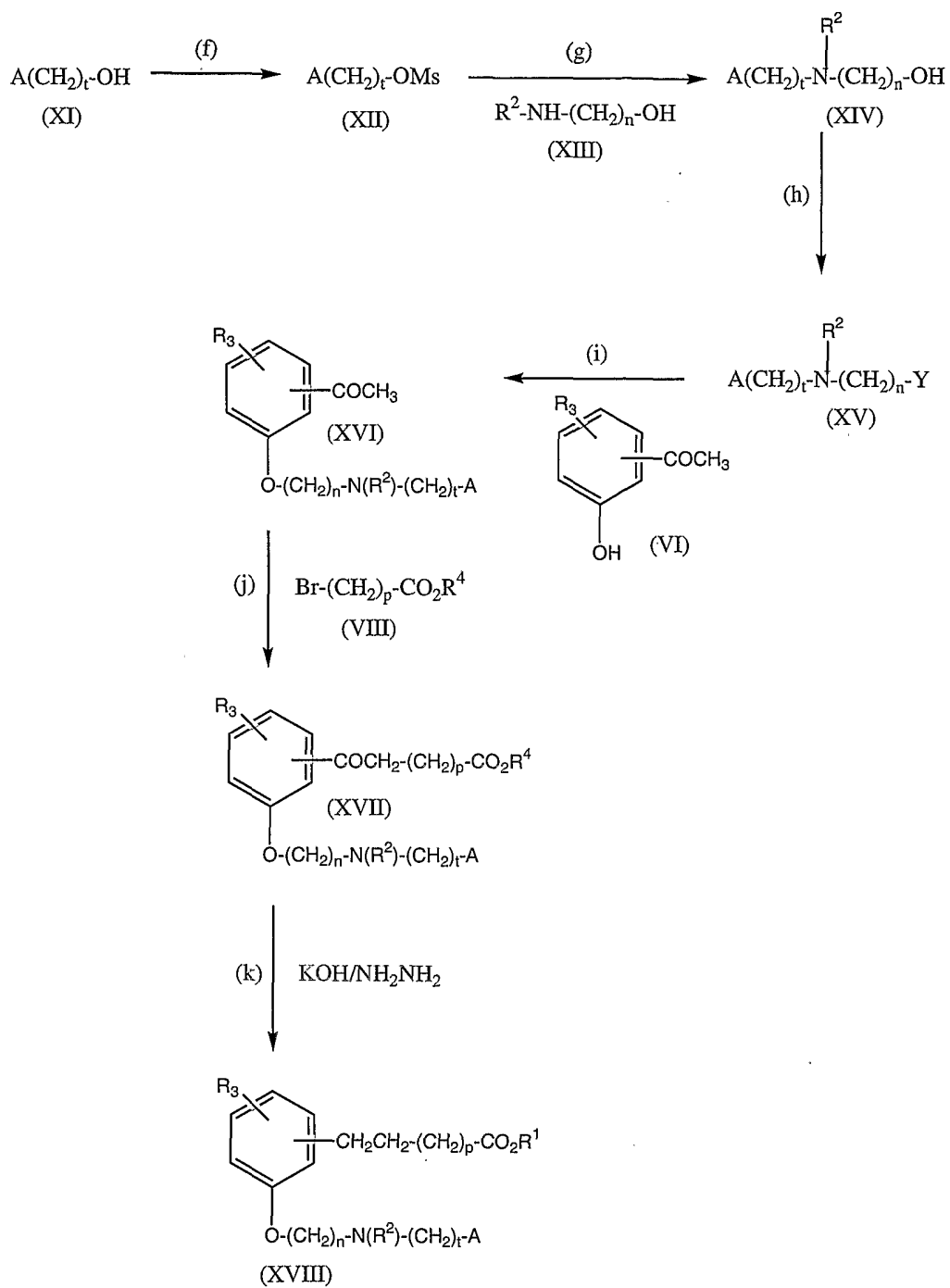
Reaction Scheme 3
