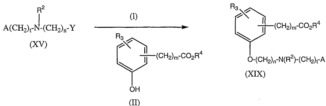
Reaction Scheme 4
