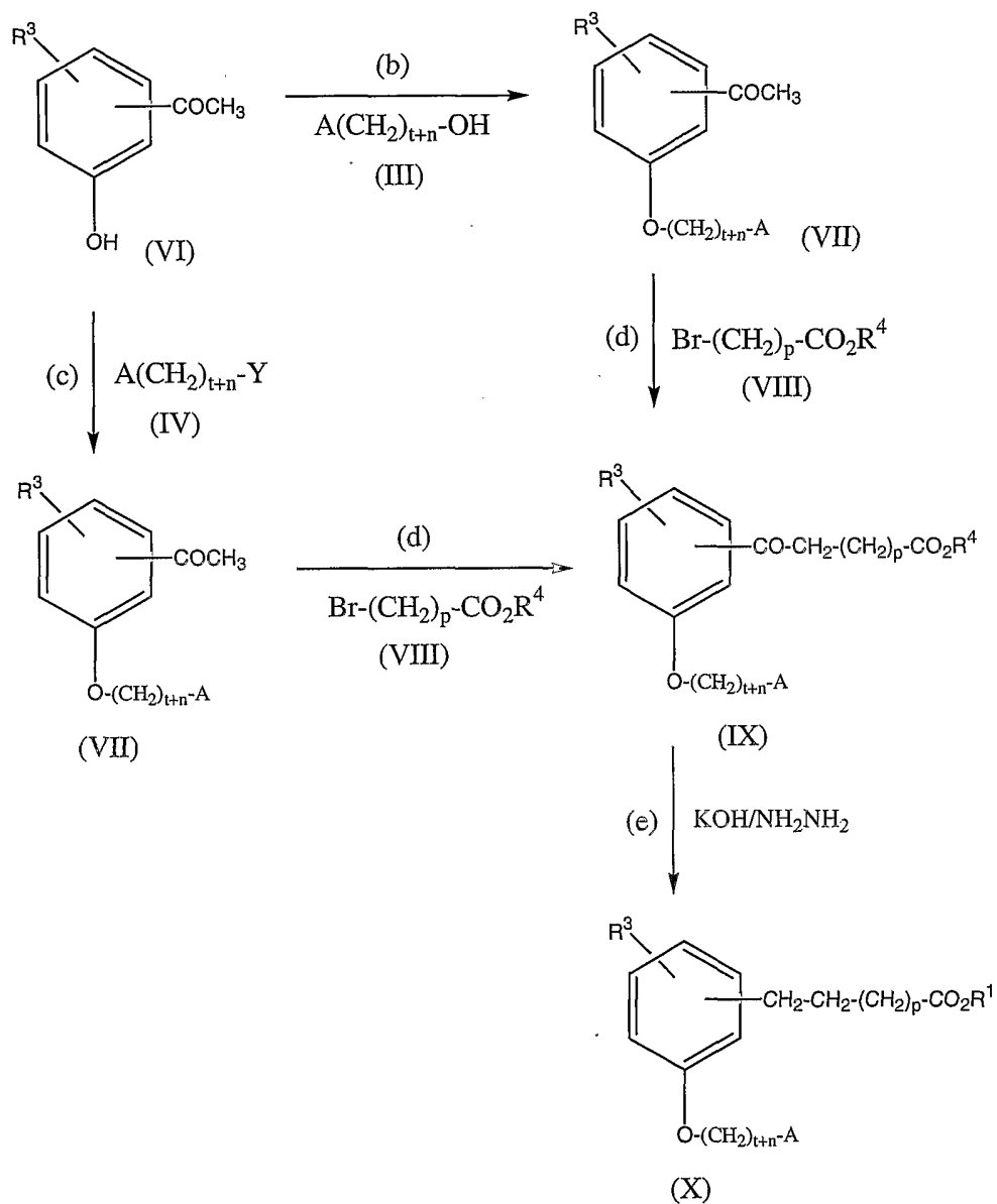
Reaction Scheme 2
