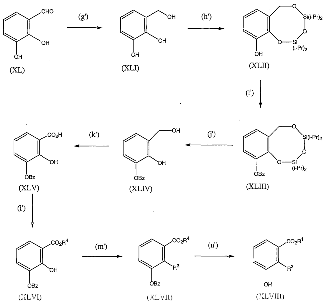
Reaction Scheme 9
