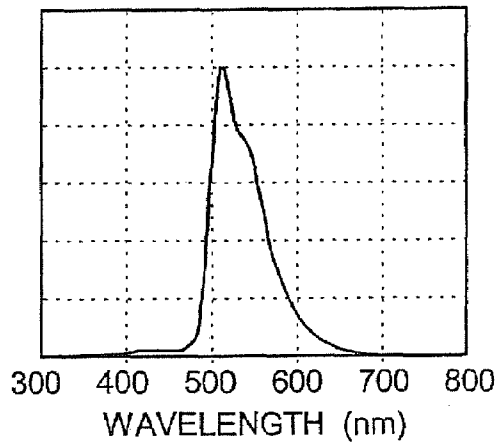
FIG. 6D LIGHT EMISSION SPECTRUM
