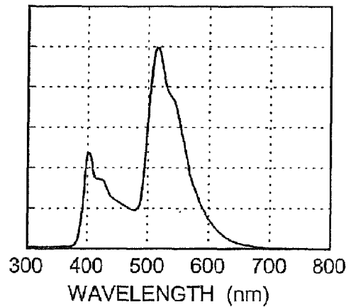
FIG. 10D LIGHT EMISSION SPECTRUM
