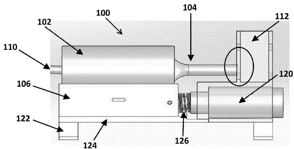
Solenoid Off
