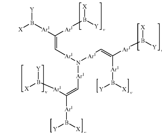
Formula (29b)
