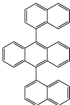
Host H
