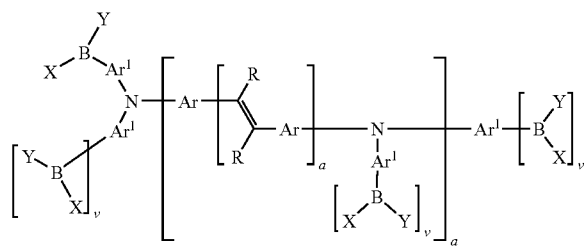
Formula (29b)
