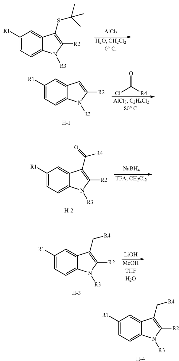
Scheme H:
