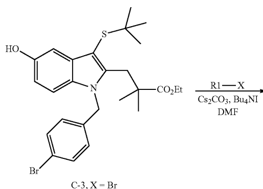
Scheme E:
