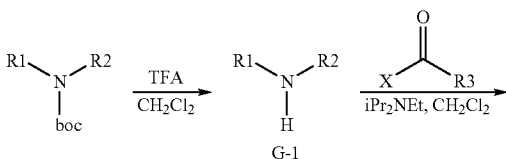
Scheme G:
