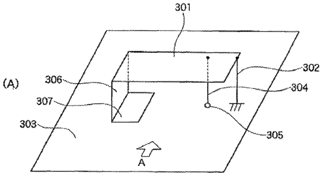
FIG. 8 PRIOR ART
