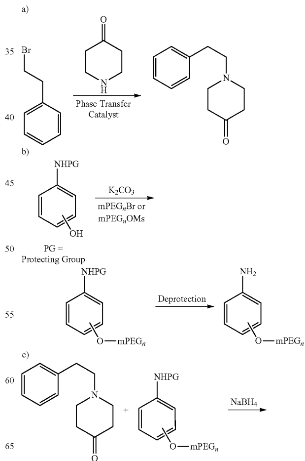
Scheme 11-C
