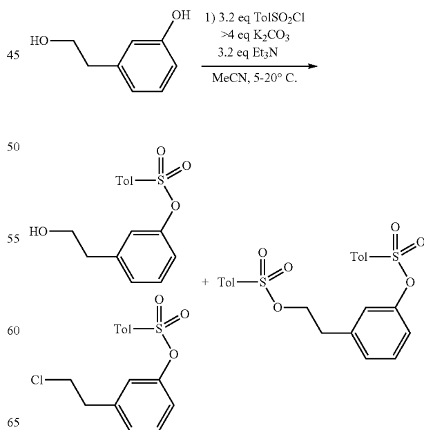
Scheme 11-B
