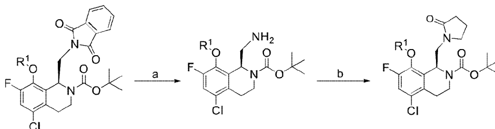
Scheme 3: a) N 2 H 4 , EtOH; b) methyl 4-bromobutanoate, Et 3 N, PhMe.
