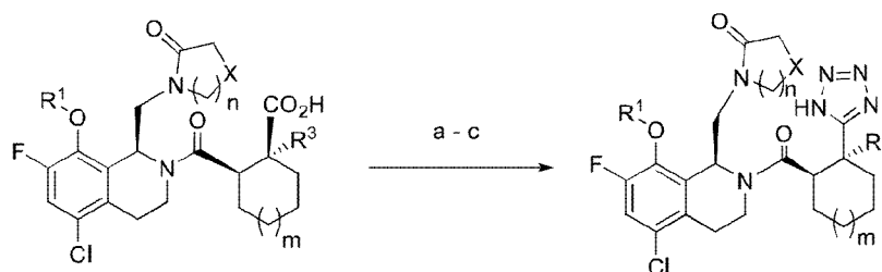
Scheme 2: a) HATU, DIPEA, NH 4 Cl, DMF; b) POCl 3 , imidazole, pyridine; c) n Bu 3 SnN 3 , xylene.
