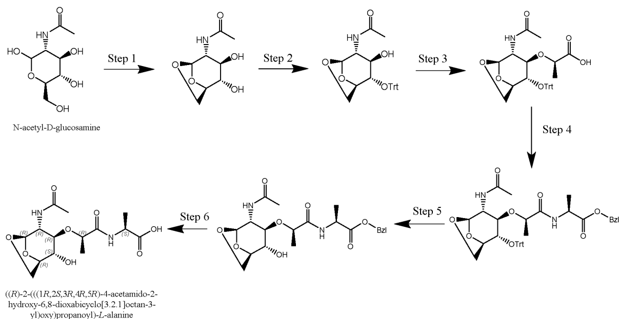
Scheme 6. Synthesis of 1,6-Anhydro- N -acetylmuramic acid- L -Alanine
