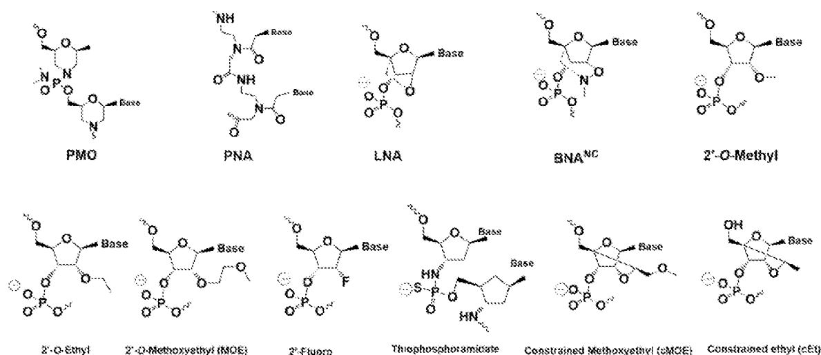
Scheme 1. Modified oligonucleotide monomer units utilised in ASO sequences
