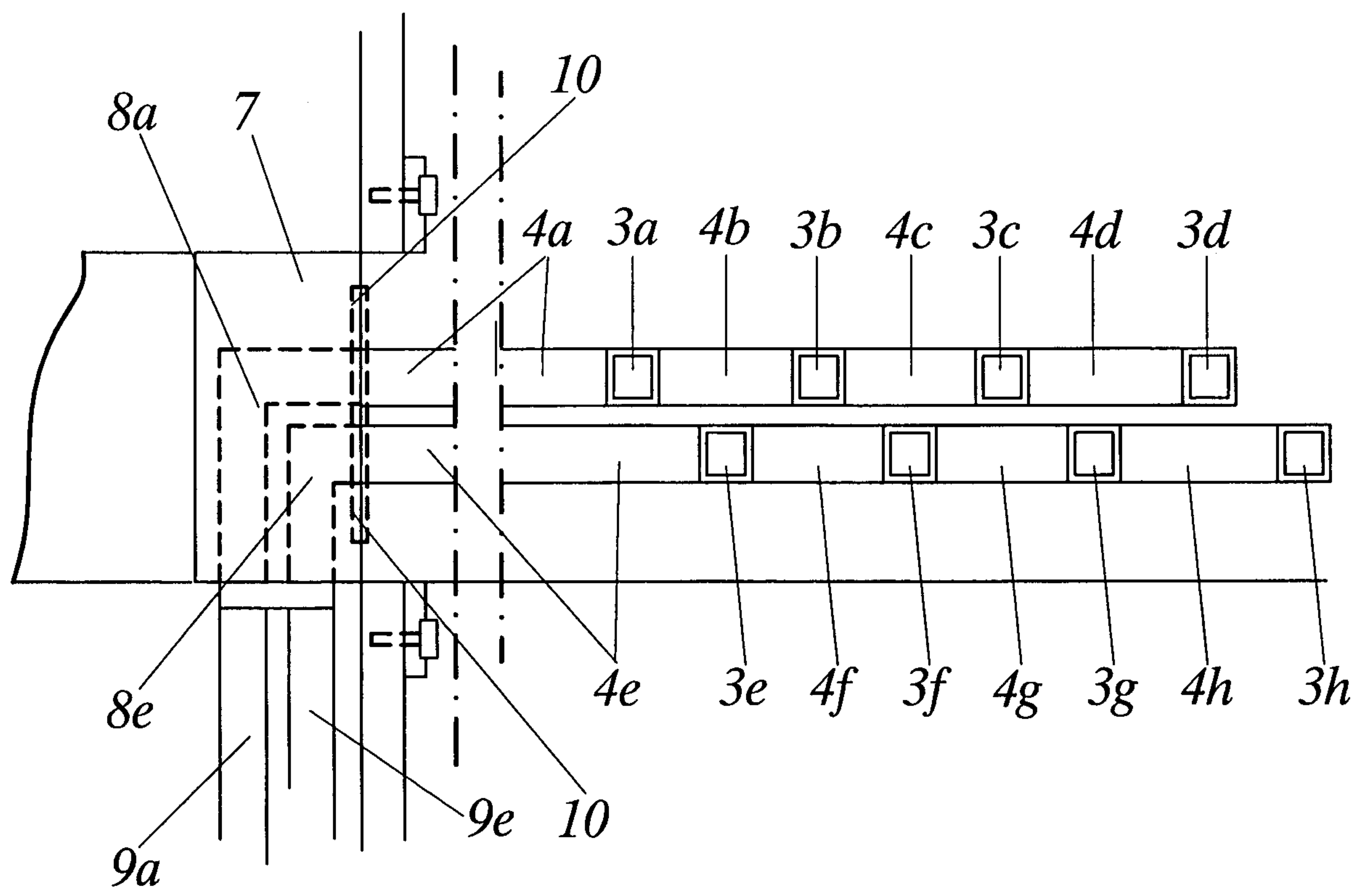
FIG. 4 (C)
