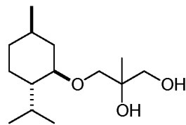
l -Menthoxo-2-methyl 1,2-propanediol
