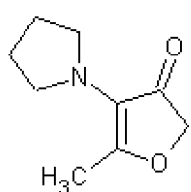
5-methyl-4-(1-pyrrolidinyl)-3-[2H]-furanone
