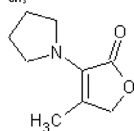
4-methyl-3-(1-pyrrolidinyl)-2[5H]-furanone
