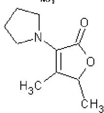
4,5-dimethyl-3-(1-pyrrolidinyl)-2[5H]-furanone
