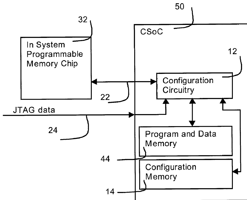
Figure 3. PRIOR ART
