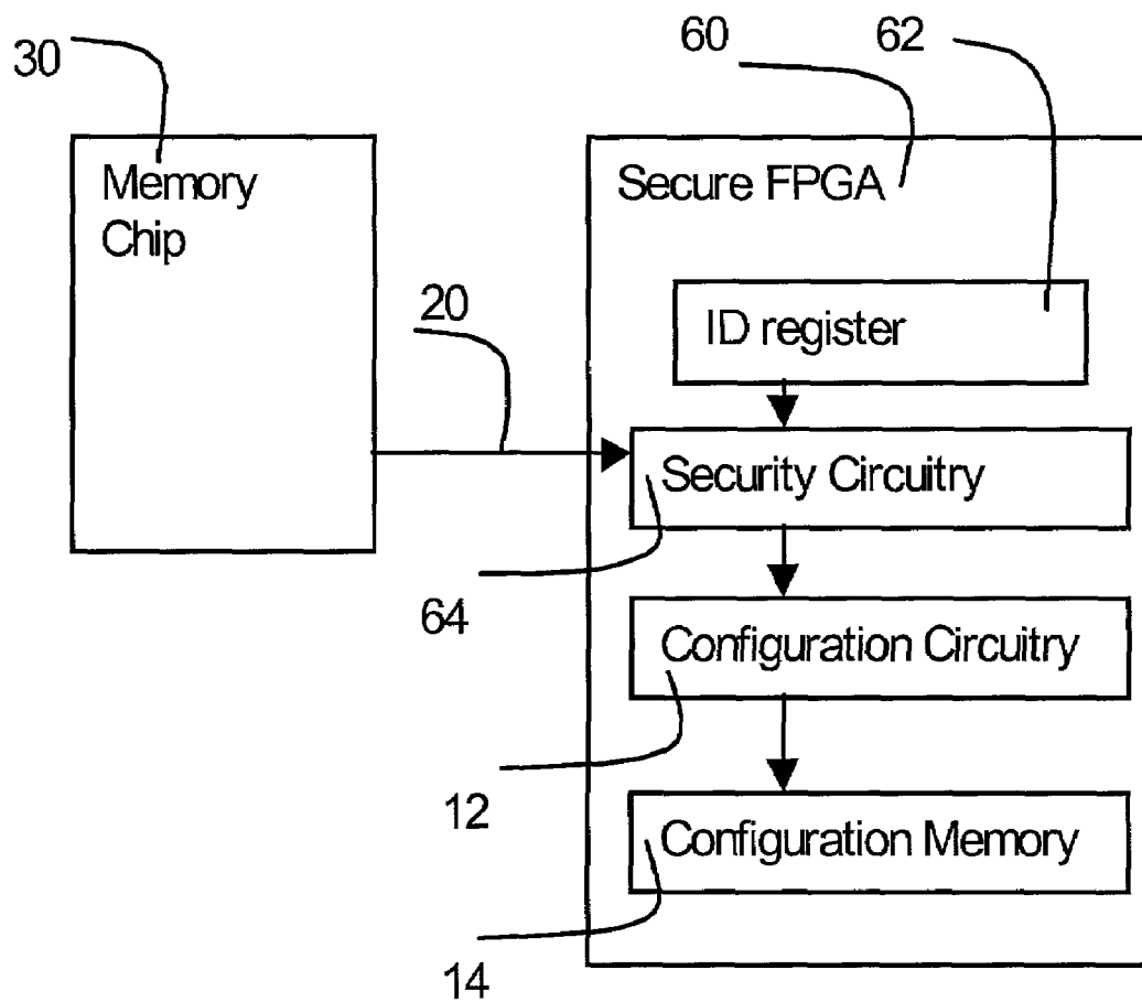
Figure 4 - PRIOR ART
