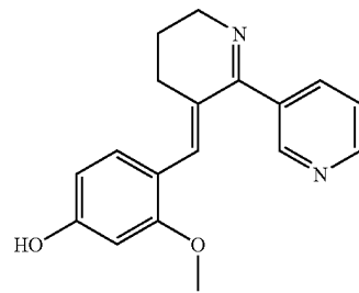
3-(4-hydroxy-2-methoxybenzylidene) anabaseine
