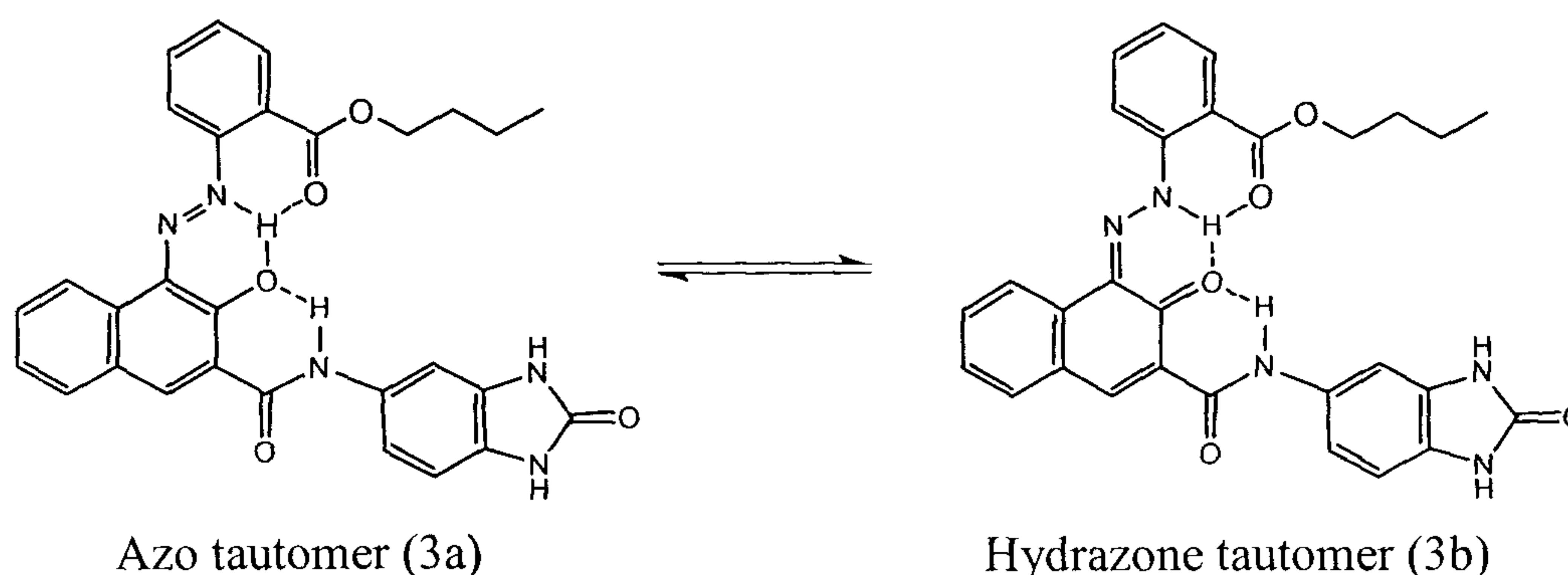
Pigment Red 208 (C.I. No. 12514)
