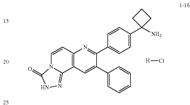
SCHEME 1B
