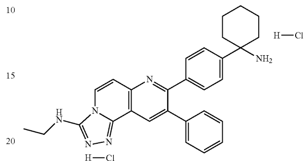
8-[4-(1-aminocyclohexyl)phenyl]-N-ethyl-9-phenyl[1,2,4]triazolo[3,4-f]-1,6-naphthyridin-3-amine dihydrochloride (6-1)
