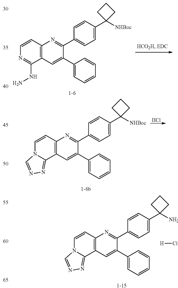
SCHEME 1B
