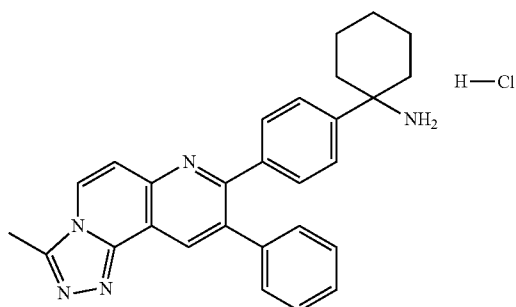
Compound 5-2
