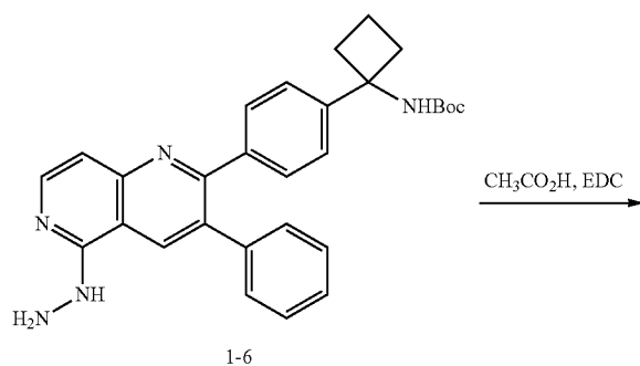
SCHEME 1F
