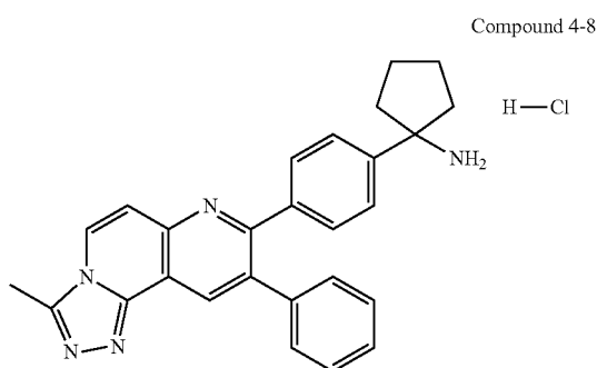
1-{4-[3-methyl-9-(4-fluorophenyl)[1,2,4]triazolo[3,4-f]-1,6-naphthyridin-8-yl]phenyl}cyclopentanamine hydrochloride (4-8)
