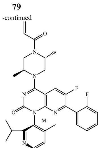
Step 1: 2,6-Dichloro-5-fluoronicotinamide (Intermediate F)
