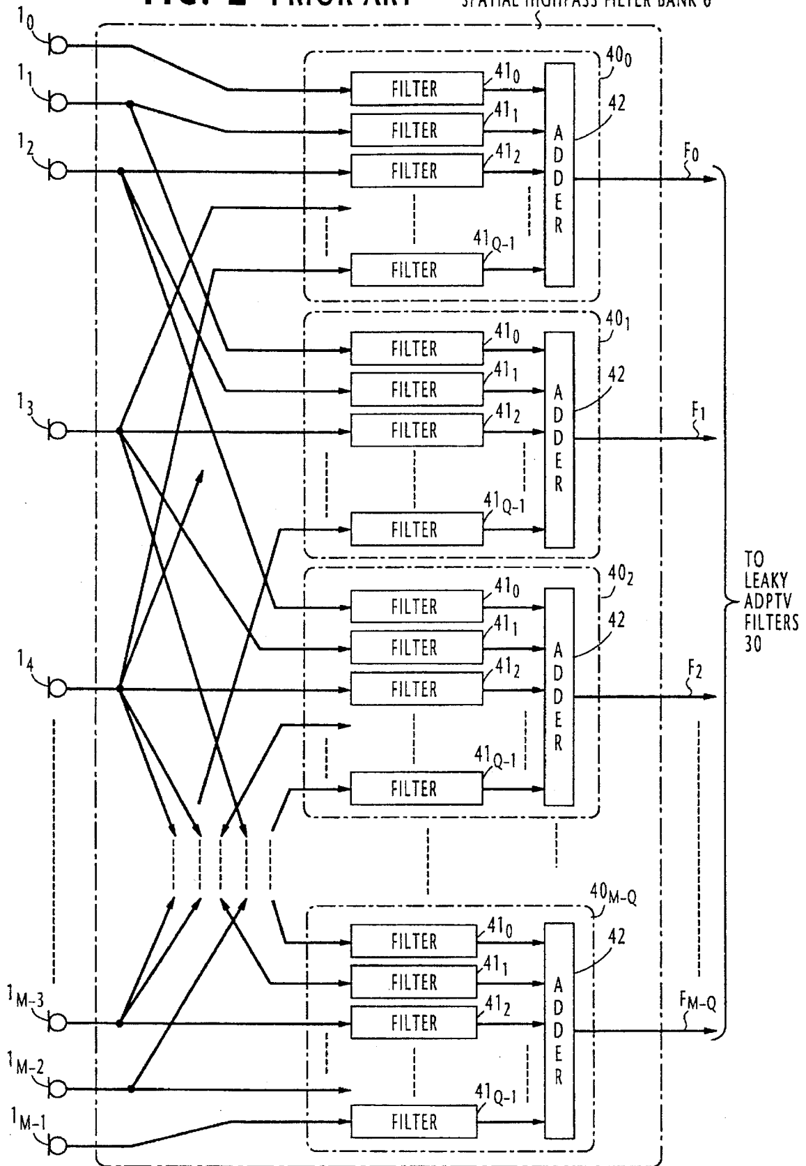
FIG. 2 PRIOR ART
