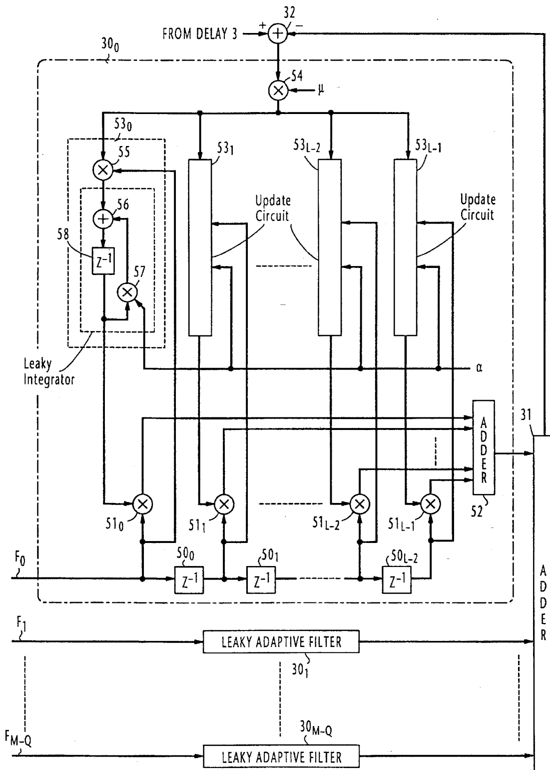
FIG. 3 PRIOR ART
