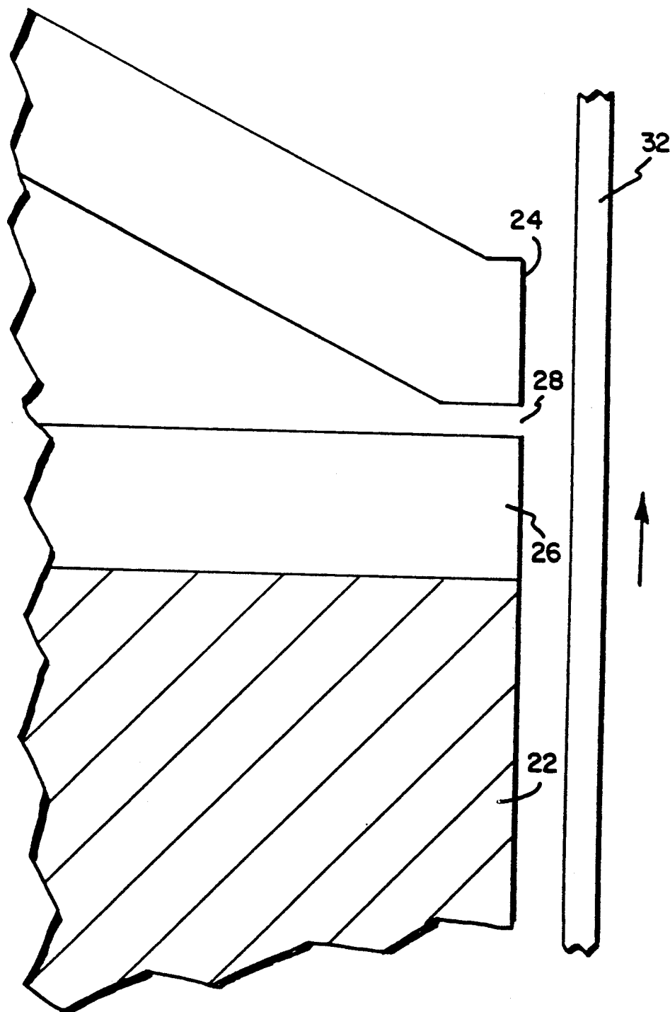
Fig. 4 PRIOR ART
