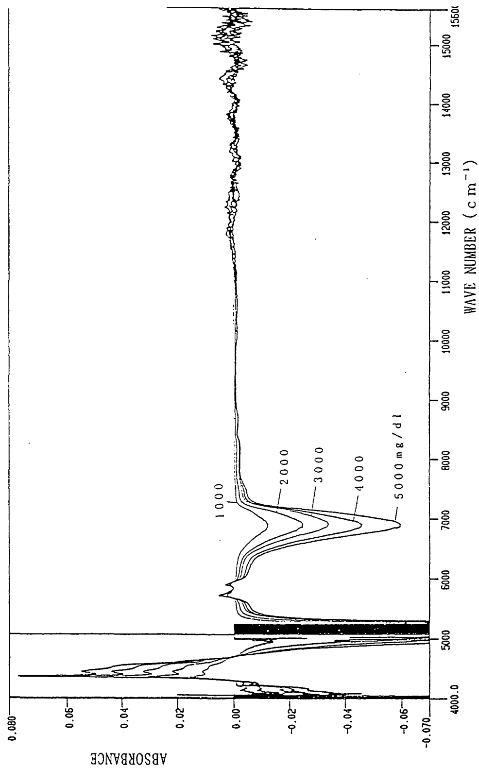
Fig. 36 SPECTRA OF AQUEOUS CREATININE SOLUTIONS
