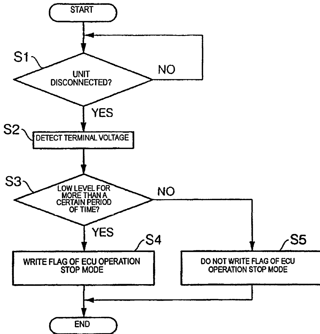
FLOWCHART WHEN ECU UNIT IS DISCONNECTED
