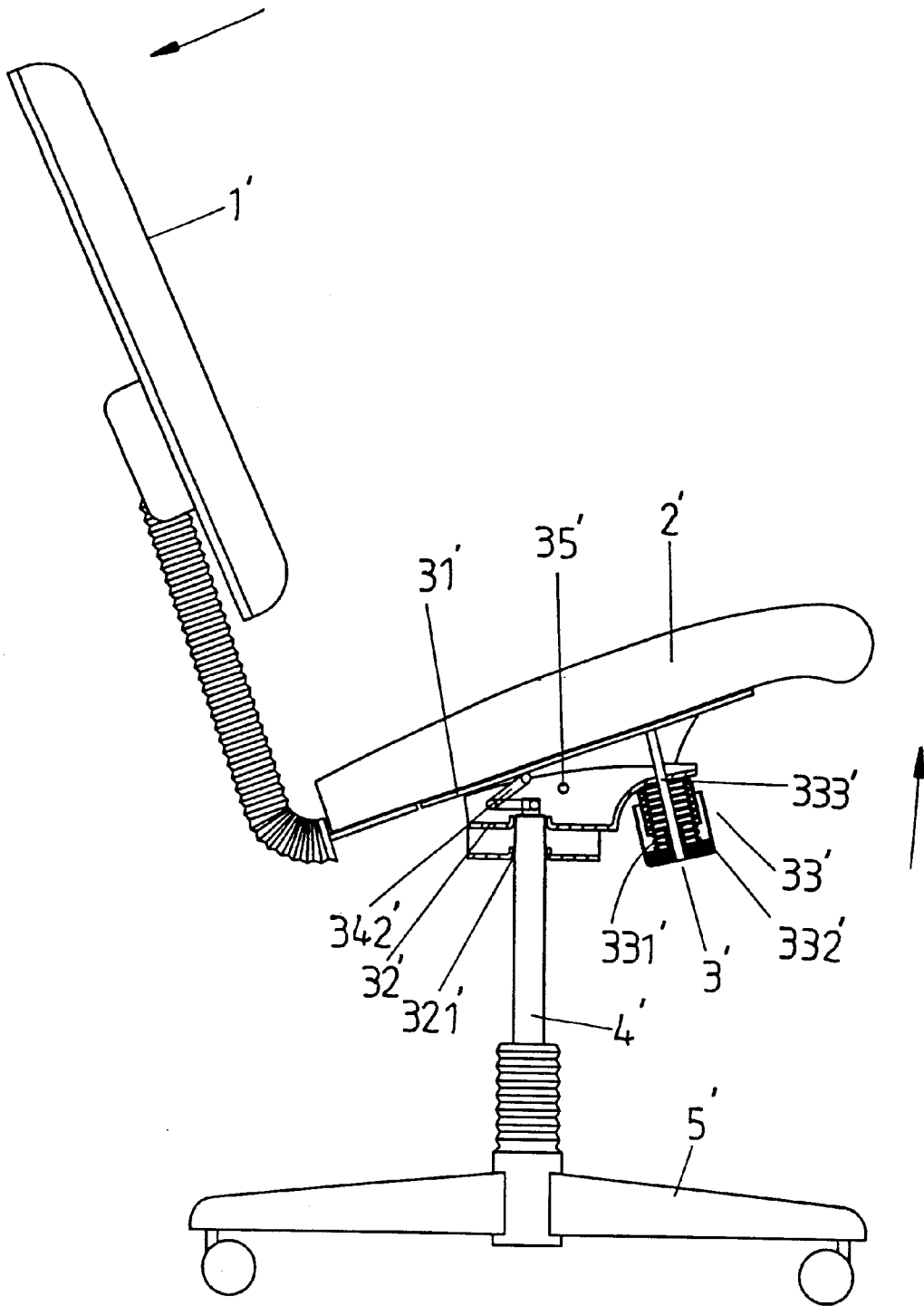
FIG. 12 Prior Art
