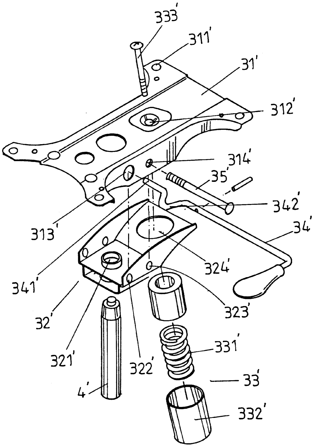
FIG. 11 Prior Art
