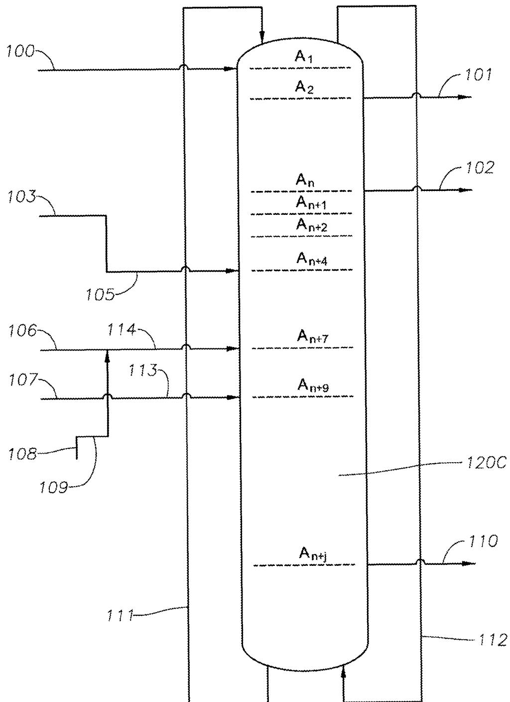
Fig. 3 (Prior Art)
