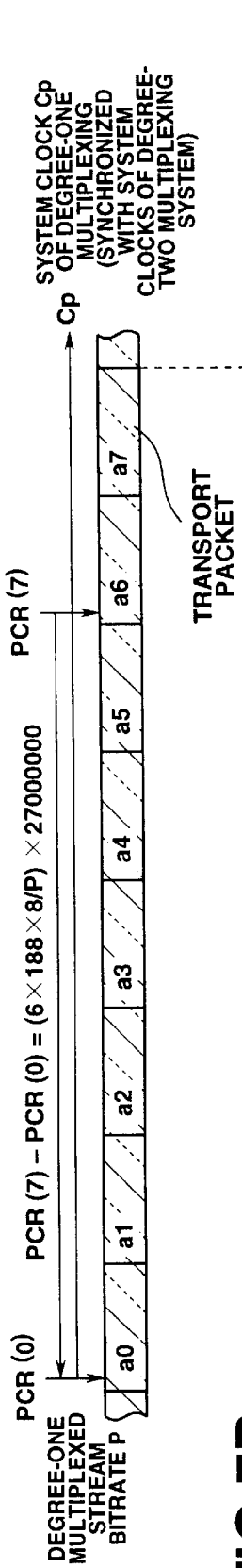
FIG. 7A (RELATED ART) IN CASE OF SYNC SYSTEM ( C_p = Cr )
