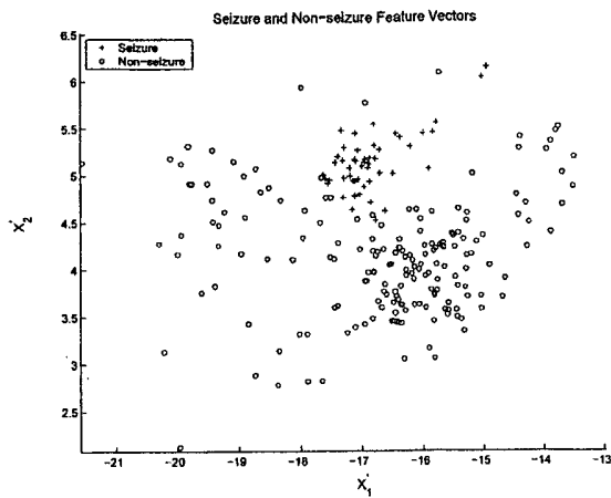
Training Seizure and Non-Seizure Feature Vectors
