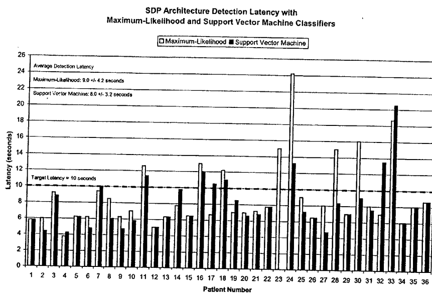
SDP Architecture Detection Latency
