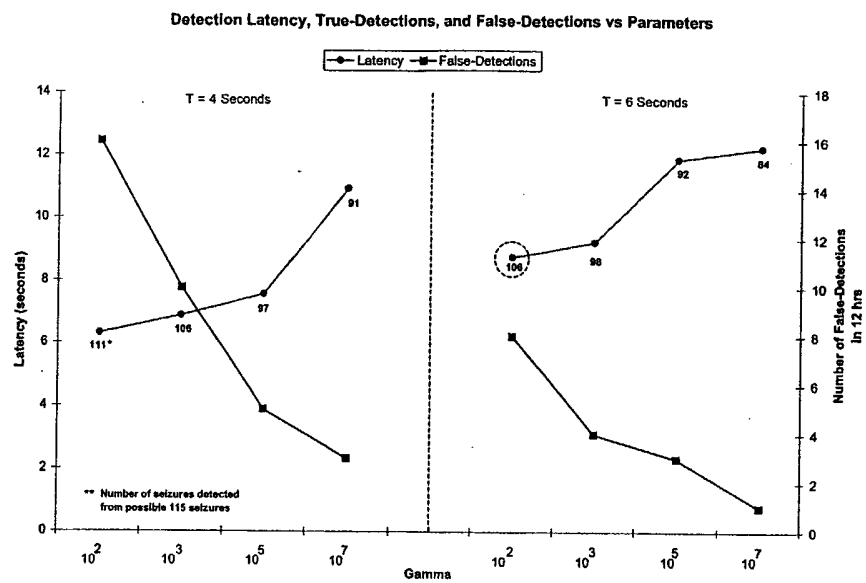
SDP Architecture Sensitivity with Maximum-Likelihood Classifier
