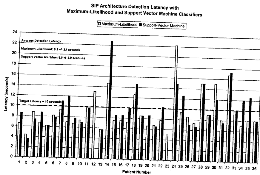
SIP Architecture Detection Latency
