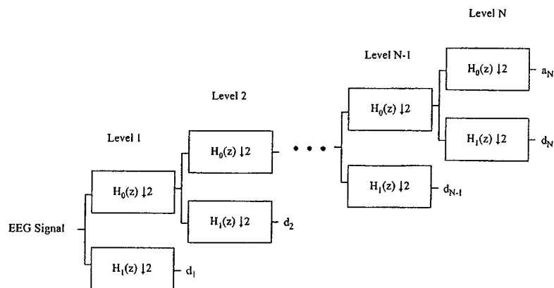
Multi-Level Wavelet Decomposition Filter Bank
