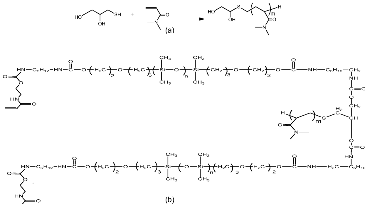
Figure 1. Schematic illustration of preparation of pDMA-pDMS macromer: (a) dihydroxy Pdma; (b) pDMA-pDMS macromer, containing multiple segments of pDMA and pDMS)... macromer, containing multiple segments of pDMA and pDMS)..
