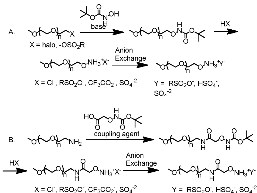
Scheme 7: Synthesis of PEG-Aminoxy reagents
