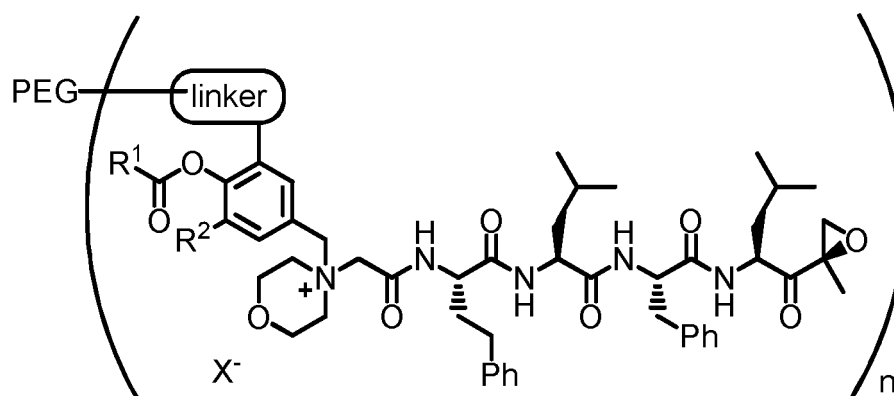
Formula II
