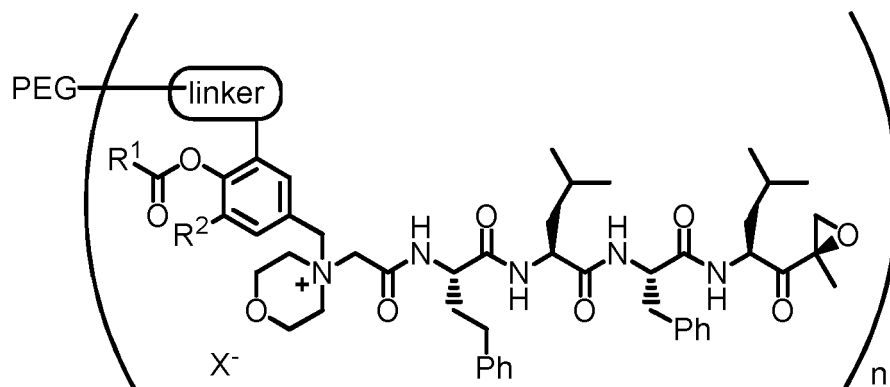
Formula II
