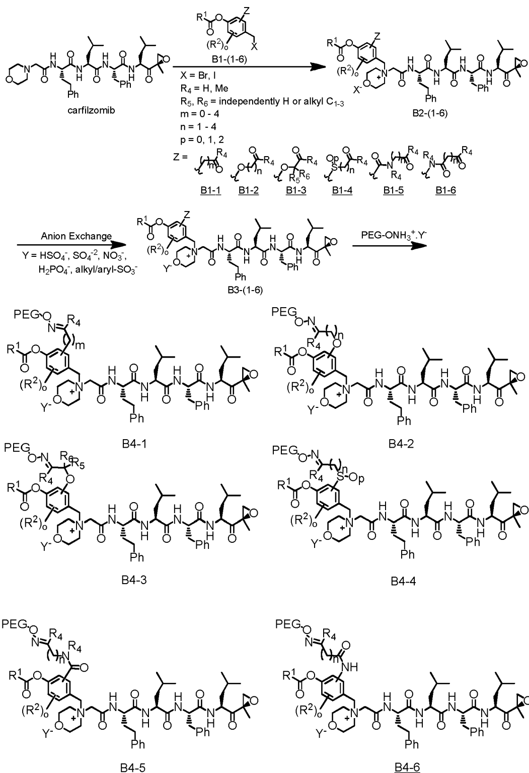
Scheme 6: Two-step polymer conjugation via aminooxy/carbonyl chemistry
