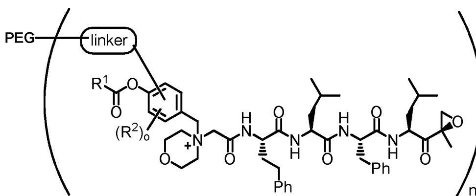
Formula I
