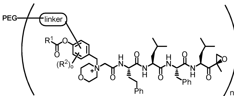
Formula I
