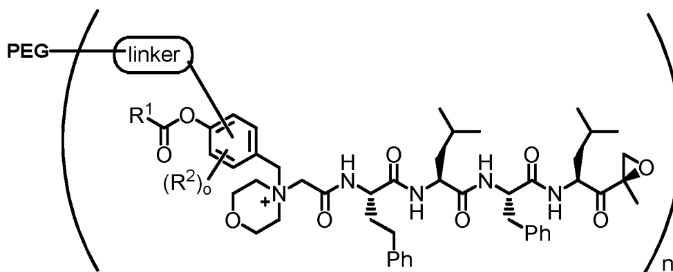
Formula I
