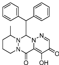
12-benzhydryl-4-hydroxy-10-methyl-7,8,9,10-tetrahydro-12H-dipyridazino[1,2-a:1',6'-d][1,2,4]triazine-3,5-dione;
