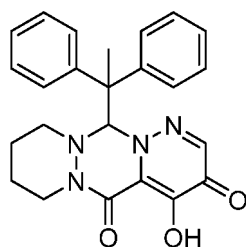
12-(1,1-diphenylethyl)-4-hydroxy-7,8,9,10-tetrahydro-12H-dipyridazino[1,2-a:1',6'-d][1,2,4]triazine-3,5-dione;
