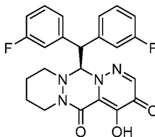
1a (R)-12-(bis(3-fluorophényl)méthyl)-4-hydroxy-7,8,9,10-tétrahydro-12H-dipyridazino[1,2-a:1',6'-d][1,2,4]triazine-3,5-dione ;
