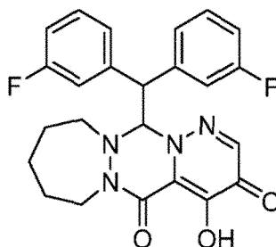
1a 13-(bis(3-fluorophényl)méthyl)-4-hydroxy-8,9,10,11-tétrahydro-7H,13H-pyridazino[1',6':4,5][1,2,4]triazino[1,2-a][1,2]diazépine-3,5-dione ;
