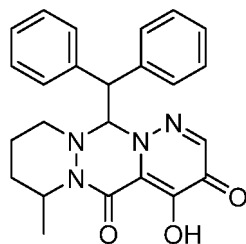
12-benzhydryl-4-hydroxy-7-methyl-7,8,9,10-tetrahydro-12H-dipyridazino[1,2-a:1',6'-d][1,2,4]triazine-3,5-dione;
