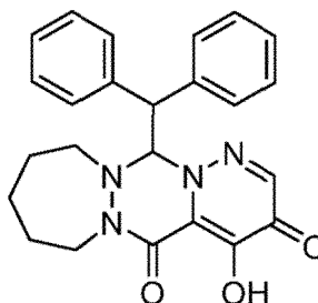
1a 13-benzhydryl-4-hydroxy-8,9,10,11-tétrahydro-7H,13H-pyridazino[1',6':4,5][1,2,4]triazino[1,2-a][1,2]diazépine-3,5-dione ;
