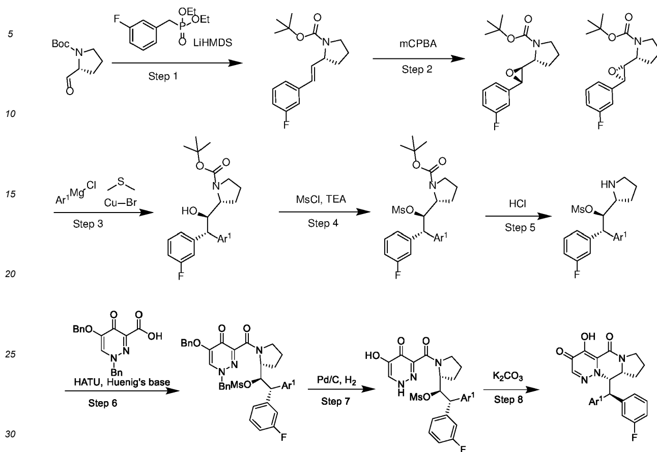
Scheme C.
