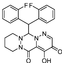
12-(bis(2-fluorophenyl)methyl)-4-hydroxy-7,8,9,10-tetrahydro-12H-dipyridazino[1,2-a:1',6'-d][1,2,4]triazine-3,5-dione;
