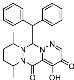
12-benzhydryl-4-hydroxy-7,10-dimethyl-7,8,9,10-tetrahydro-12H-dipyridazino[1,2-a:1',6'-d][1,2,4]triazine-3,5-dione;
