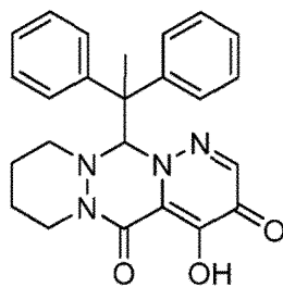
1a 12-(1,1-diphényléthyl)-4-hydroxy-7,8,9,10-tétrahydro-12H-dipyridazino[1,2-a:1',6'-d][1,2,4]triazine-3,5-dione ;
