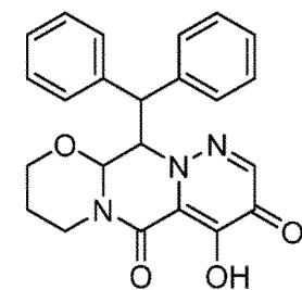
1a 12-benzhydryl-7-hydroxy-3,4,12,12a-tétrahydro-2H-pyridazino[1',6':4,5]pyrazino[2,1-b][1,3]oxazine-6,8-dione ;
