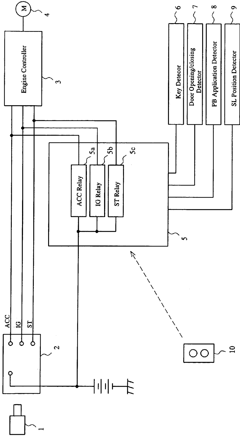
Fig.11 PRIOR ART
