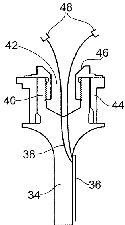
FIG. 1 (Prior Art)
